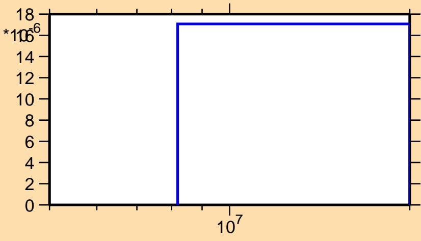
\sigma vs. E for ^{200}\text{Ir}(n,d)
