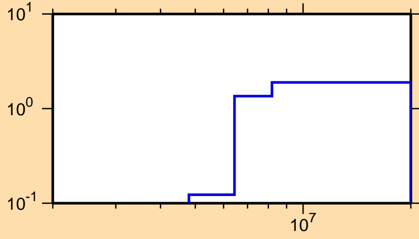
\sigma vs. E for ^{200}\text{Ir}(n,2n)
