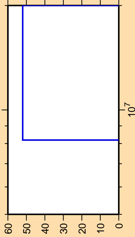
\Delta\sigma/\sigma vs. E for ^{200}\text{Ir}(n,np)
