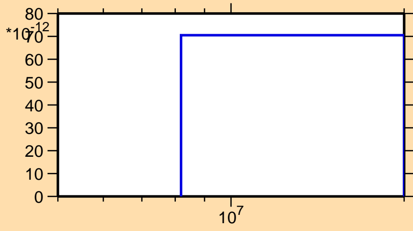
\sigma vs. E for ^{200}\text{Ir}(n,2np)
