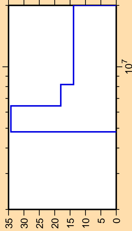
\Delta\sigma/\sigma vs. E for ^{200}\text{Ir}(n,2n)
