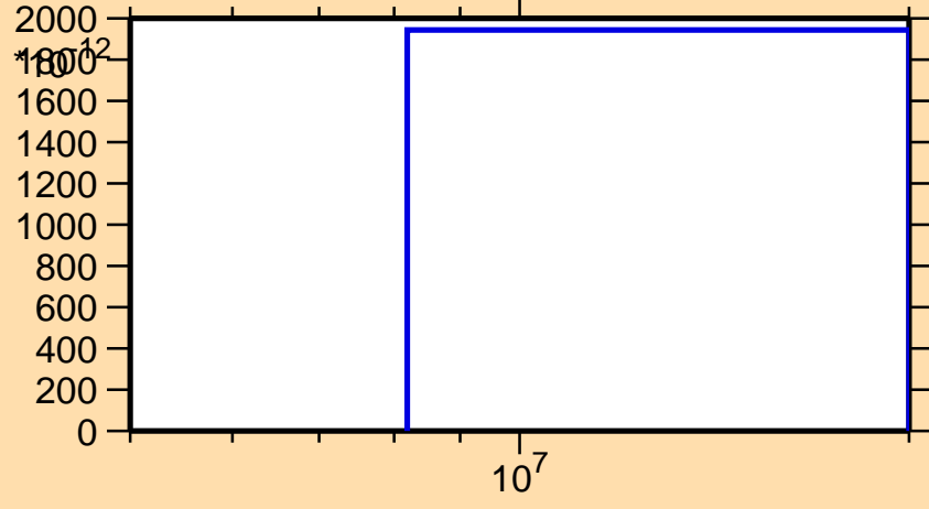
\sigma vs. E for ^{200}\text{Ir}(n,\text{nd})
