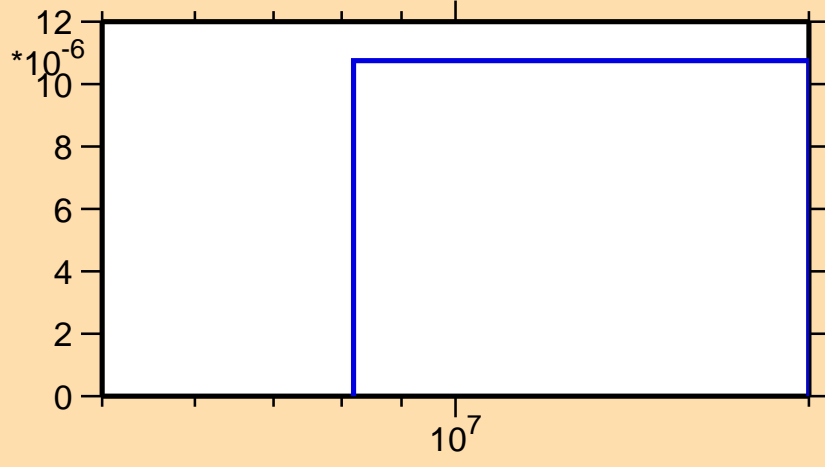
\sigma vs. E for ^{200}\text{Ir}(n,np)
