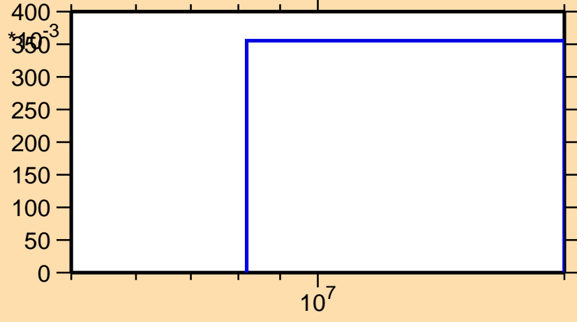
\sigma vs. E for ^{200}\text{Ir}(n,3n)
