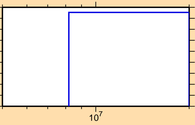
\sigma vs. E for ^{200}\text{Ir}(n,d)
