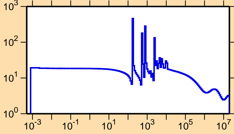
\sigma vs. E for ^{201}\text{Ir}(n,\text{el.})
