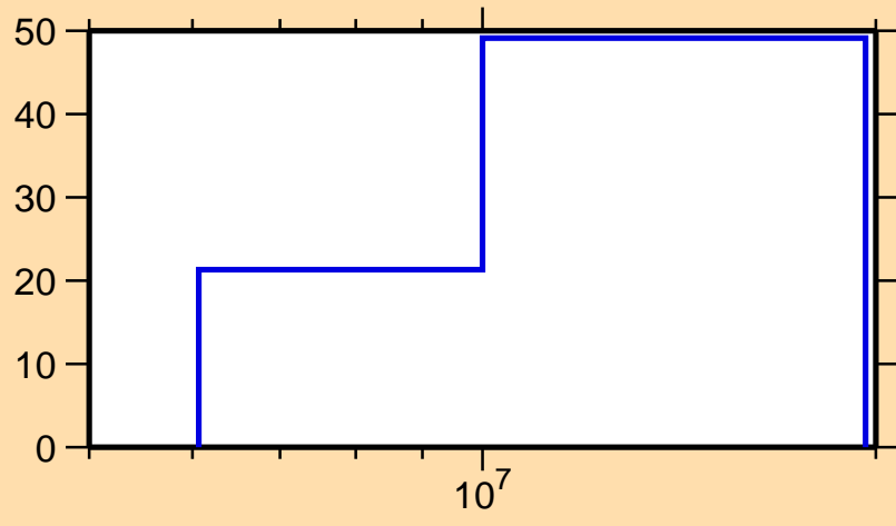
\Delta\sigma/\sigma vs. E for ^{201}\text{Ir}(n,ncont.)
