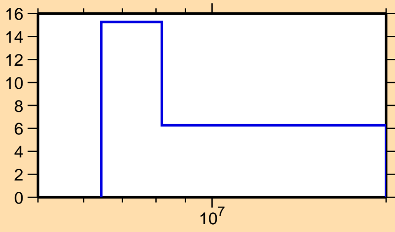
\Delta\sigma/\sigma vs. E for ^{201}\text{Ir}(n,el.)
