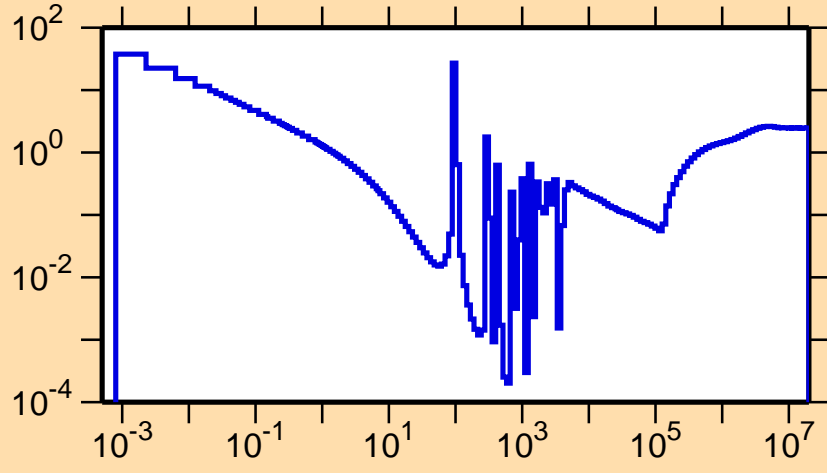
\sigma vs. E for ^{202}\text{Ir}(n,\text{nonel.})
