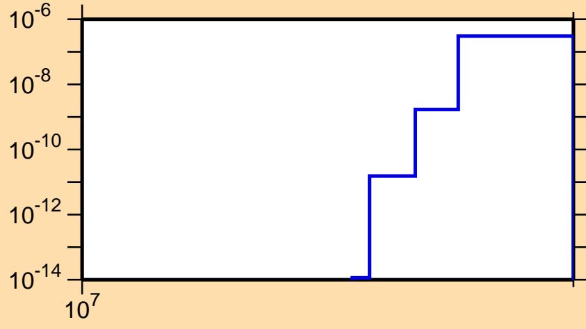
\sigma vs. E for ^{202}\text{Ir}(n,nt)
