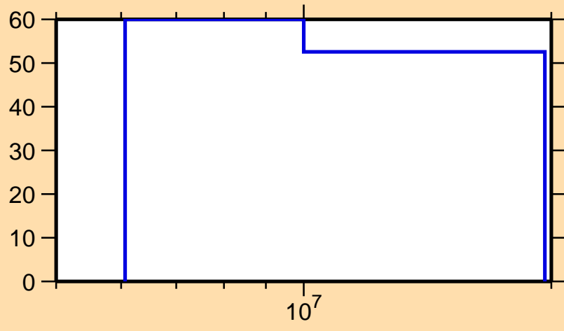
\Delta\sigma/\sigma vs. E for ^{202}\text{Ir}(n,p)
