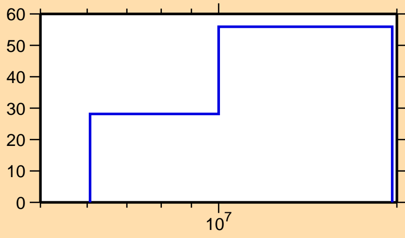
\Delta\sigma/\sigma vs. E for ^{202}\text{Ir}(n,n\text{cont.})
