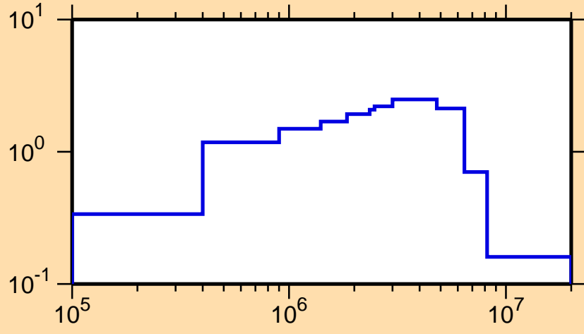
\sigma vs. E for ^{202}\text{Ir}(n,\text{inel.})
