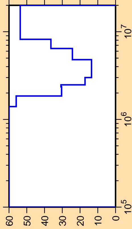
\Delta\sigma/\sigma vs. E for ^{202}\text{Ir}(n,\text{inel.})
