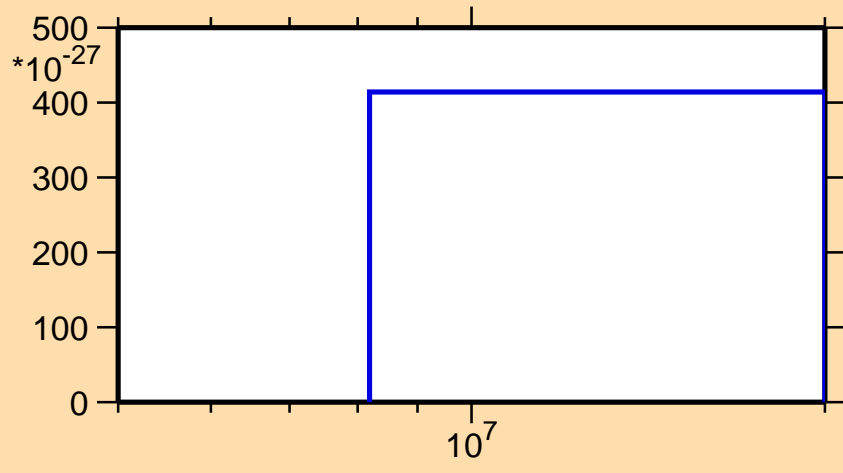
\sigma vs. E for ^{203}\text{Ir}(\text{mt } 42)
