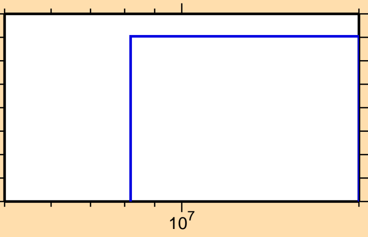
\sigma vs. E for ^{203}\text{Ir}(n,2n\alpha)
