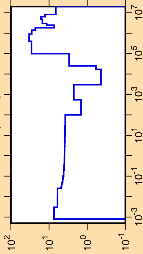
\Delta\sigma/\sigma vs. E for ^{203}\text{Ir}(n,\text{tot.})
