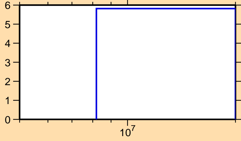
\Delta\sigma/\sigma vs. E for ^{203}\text{Ir}(n,el.)
