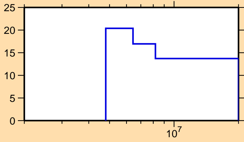
\Delta\sigma/\sigma vs. E for ^{203}\text{Ir}(n,2n)
