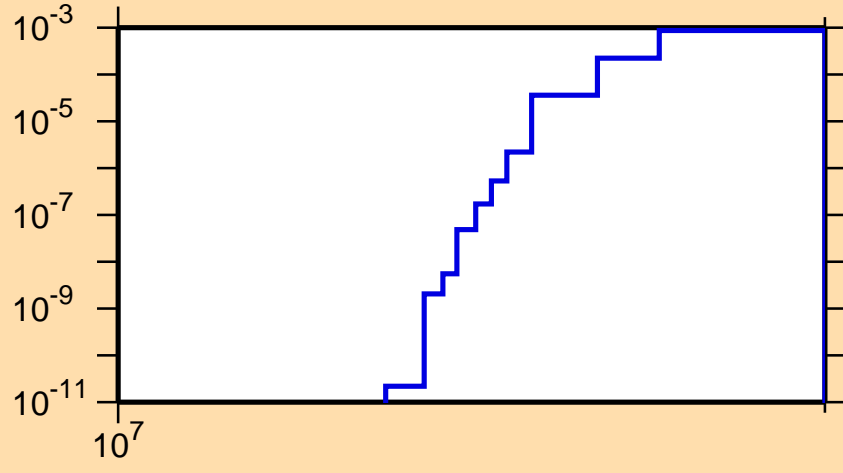
\sigma vs. E for ^{38}\text{K}(n,\text{pd})
