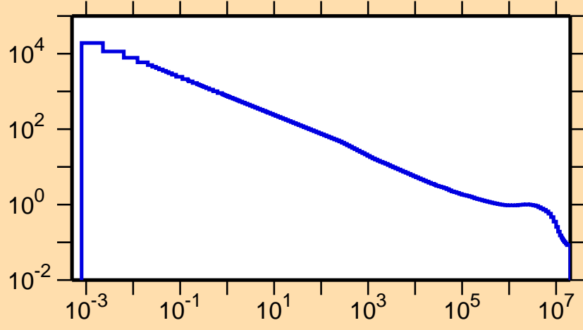
\sigma vs. E for ^{38}\text{K}(n,p)
