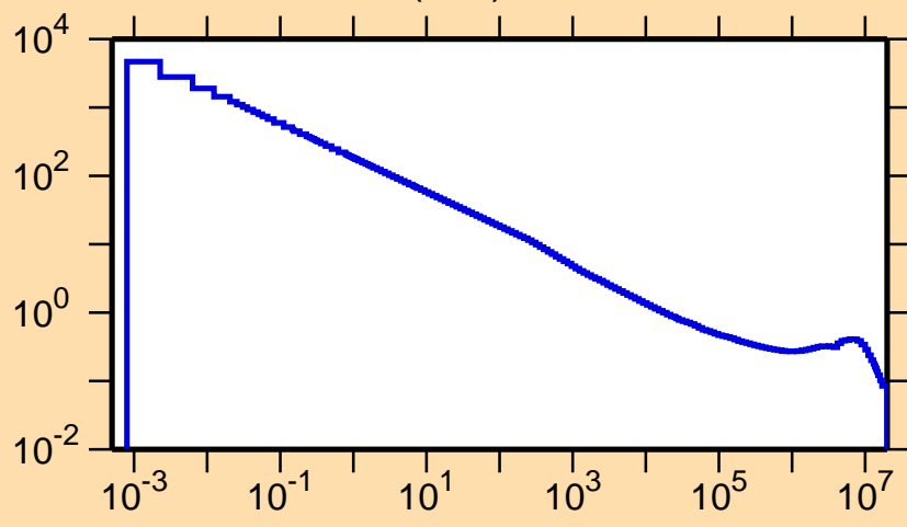
\sigma vs. E for ^{38}\text{K}(n,\alpha)
