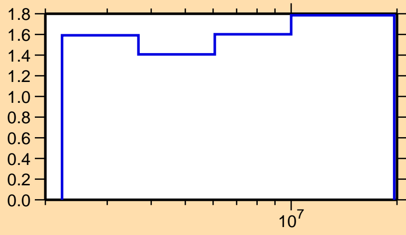
\Delta\sigma/\sigma vs. E for ^{38}\text{K}(n,n\text{onel.})
