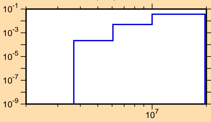
\sigma vs. E for ^{38}\text{K}(n,d)
