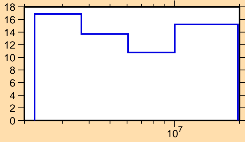
\Delta\sigma/\sigma vs. E for ^{38}\text{K}(n,n\text{cont.})
