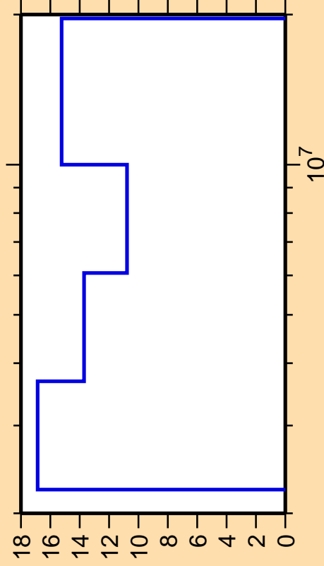
\Delta\sigma/\sigma vs. E for ^{38}\text{K}(n,ncont.)
