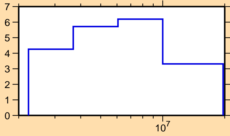
\Delta\sigma/\sigma vs. E for ^{38}\text{K}(n,el.)
