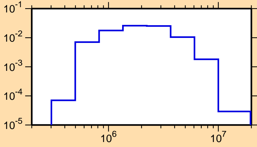
\sigma vs. E for ^{38}\text{K}(n,n_2)
