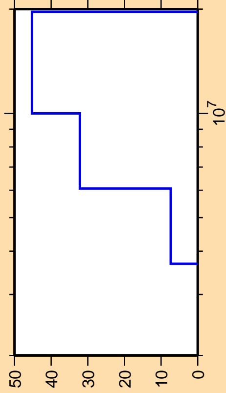
\Delta\sigma/\sigma vs. E for ^{40}\text{K}(n,d)
