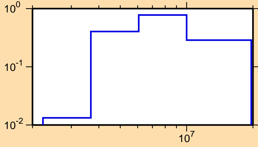
\sigma vs. E for ^{40}\text{K}(n,n\text{cont.})
