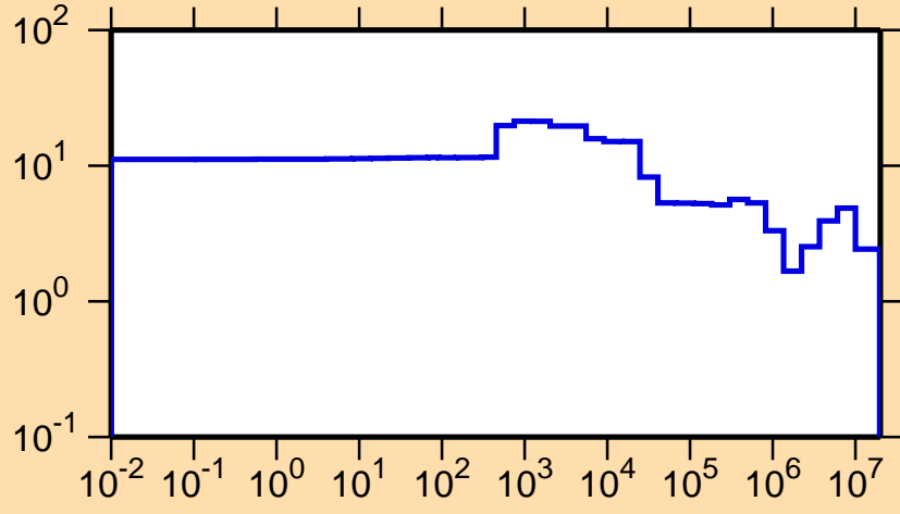
\Delta\sigma/\sigma vs. E for ^{40}\text{K}(n,el.)
