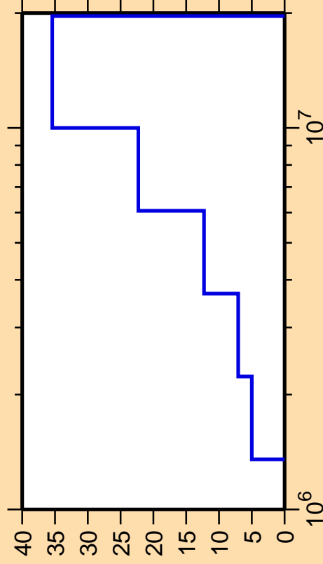
\Delta\sigma/\sigma vs. E for ^{40}\text{K}(n,n_4)
