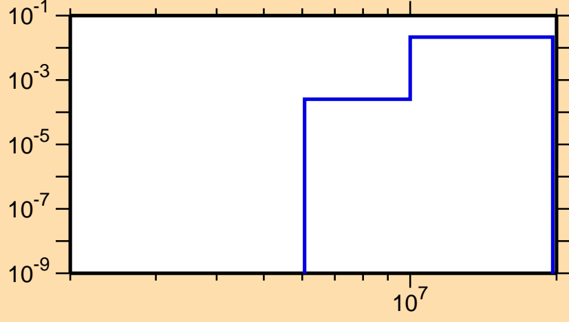
\sigma vs. E for ^{40}\text{K}(n,d)
