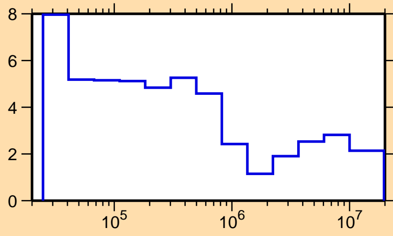
\Delta\sigma/\sigma vs. E for ^{40}\text{K}(n,\text{tot.})
