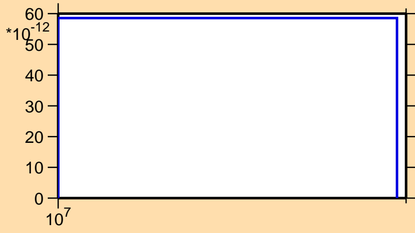
\sigma vs. E for ^{40}\text{K}(n,nt)
