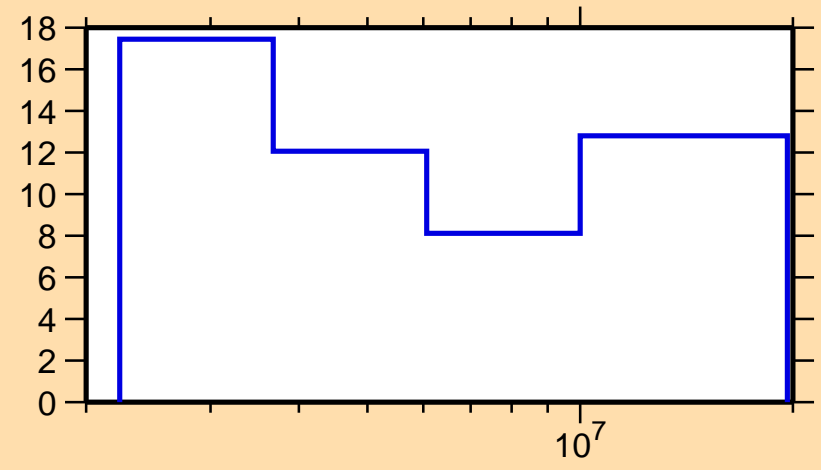
\Delta\sigma/\sigma vs. E for ^{40}\text{K}(n,ncont.)
