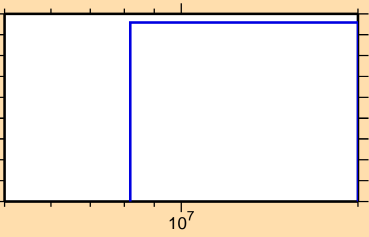
\sigma vs. E for ^{40}\text{K}(\text{mt117})
