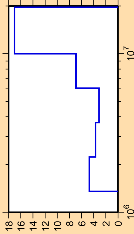
\Delta\sigma/\sigma vs. E for ^{41}\text{K}(n,n_3)
