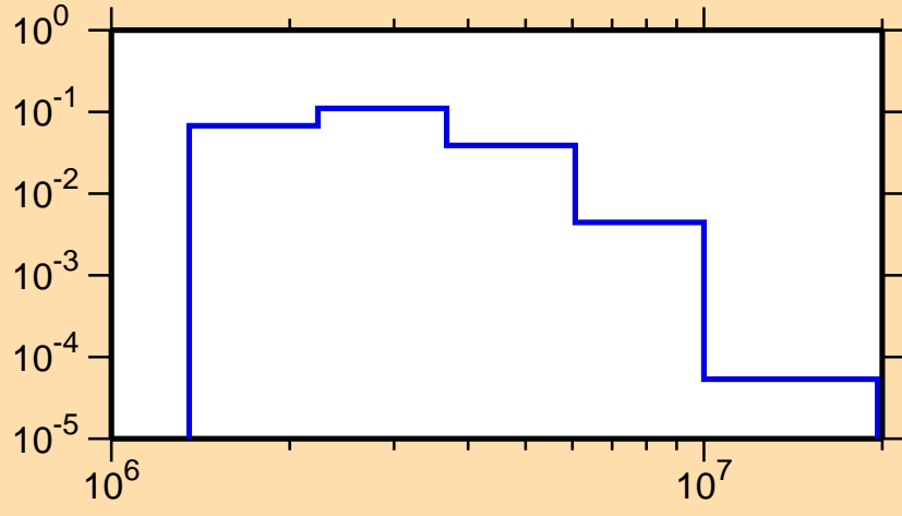
\sigma vs. E for ^{41}\text{K}(n,n_3)
