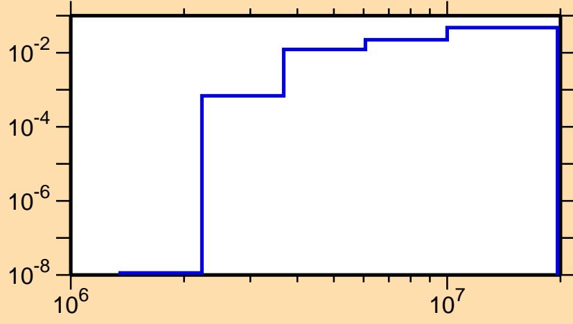
\sigma vs. E for ^{41}\text{K}(n,p)
