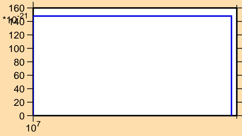
\sigma vs. E for ^{41}\text{K}(n,\text{pd})
