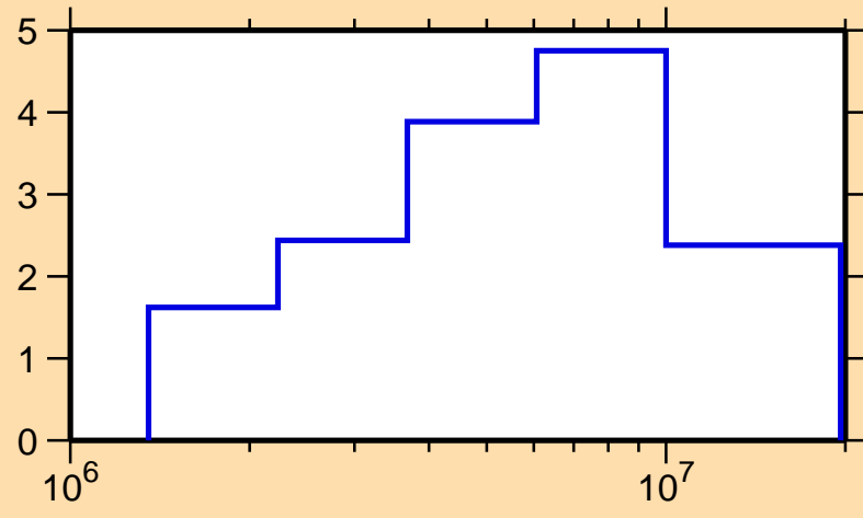
\Delta\sigma/\sigma vs. E for ^{41}\text{K}(n,el.)
