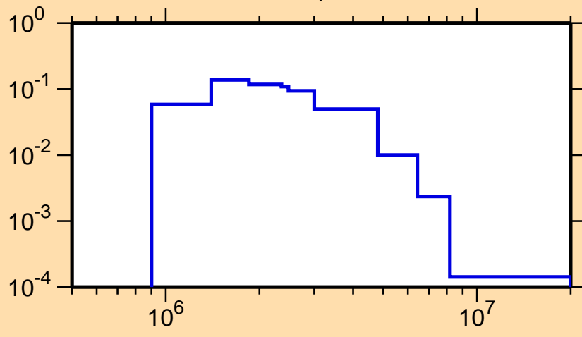
\sigma vs. E for ^{41}\text{K}(n,n_1)
