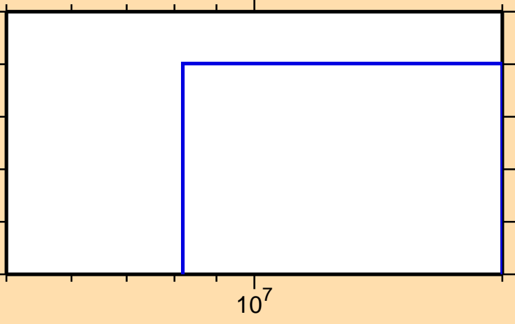
\sigma vs. E for ^{41}\text{K}(n,nt)
