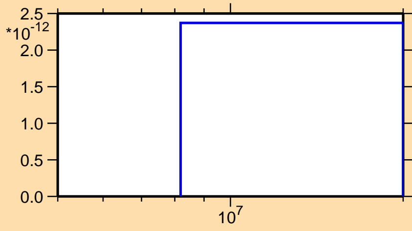
\sigma vs. E for ^{41}\text{K}(n,2n\alpha)
