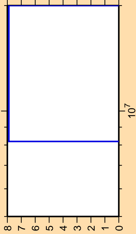
\Delta\sigma/\sigma vs. E for ^{41}\text{K}(n,\alpha)
