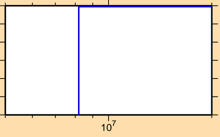
\sigma vs. E for ^{41}\text{K}(n,\text{He}3)
