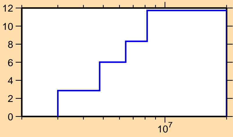
\Delta\sigma/\sigma vs. E for ^{41}\text{K}(n,n_1)
