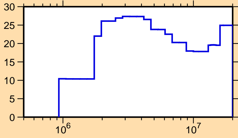
\Delta\sigma/\sigma vs. E for ^{42}\text{K}(n,p)
