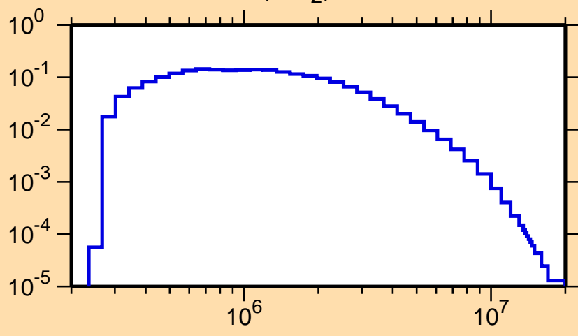
\sigma vs. E for ^{42}\text{K}(n,n_2)
