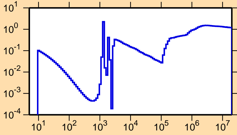
\sigma vs. E for ^{42}\text{K}(n,\text{nonel.})
