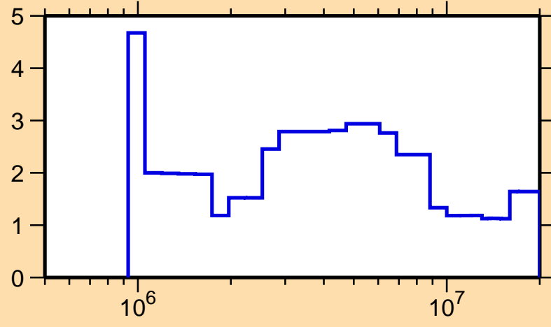
\Delta\sigma/\sigma vs. E for ^{42}\text{K}(n,\text{tot.})
