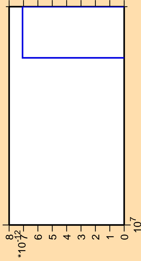
\Delta\sigma/\sigma vs. E for ^{42}\text{K}(n,\text{pt})
