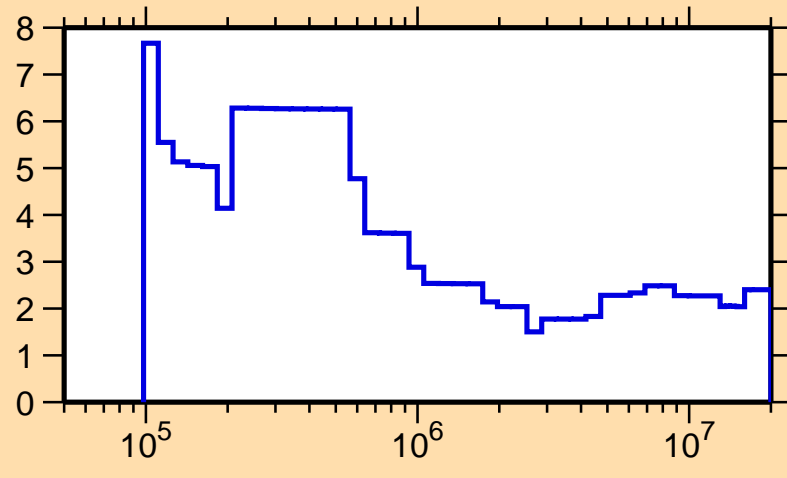
\Delta\sigma/\sigma vs. E for ^{42}\text{K}(n,\text{nonel.})
