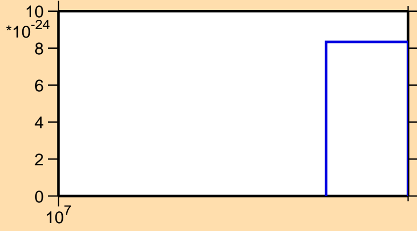
\sigma vs. E for ^{42}\text{K}(n,\text{pt})
