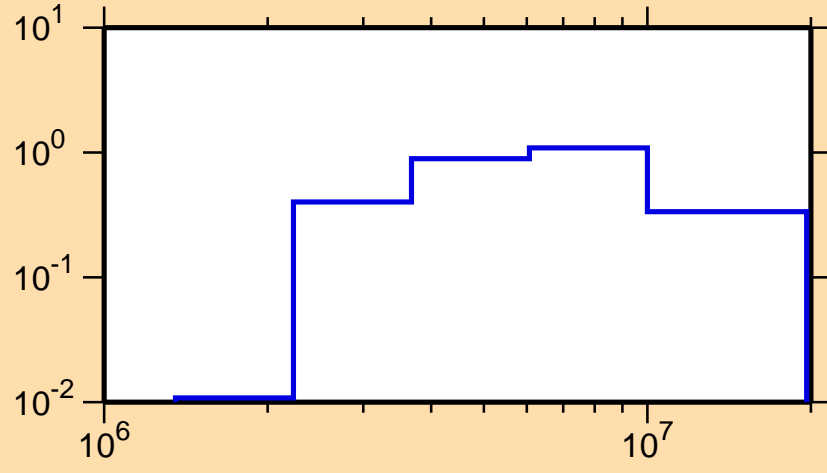
\sigma vs. E for ^{42}\text{K}(n,n\text{cont.})
