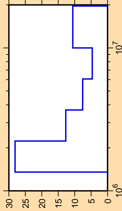
\Delta\sigma/\sigma vs. E for ^{42}\text{K}(n,ncont.)
