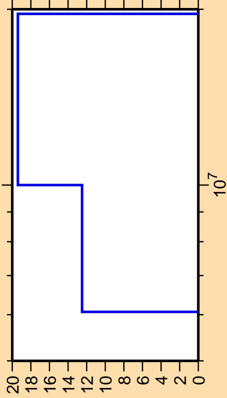
\Delta\sigma/\sigma vs. E for ^{42}\text{K}(n,d)
