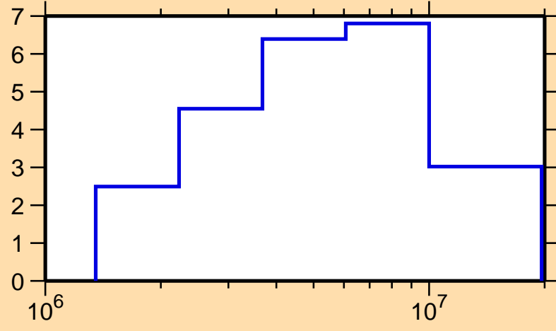
\Delta\sigma/\sigma vs. E for ^{42}\text{K}(n,el.)
