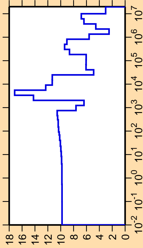
\Delta\sigma/\sigma vs. E for ^{42}\text{K}(n,\text{el.})
