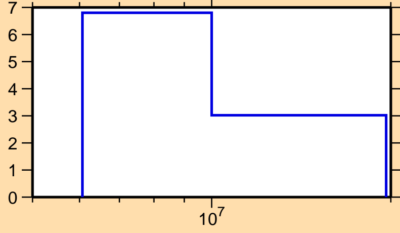
\Delta\sigma/\sigma vs. E for ^{42}\text{K}(n,\text{el.})
