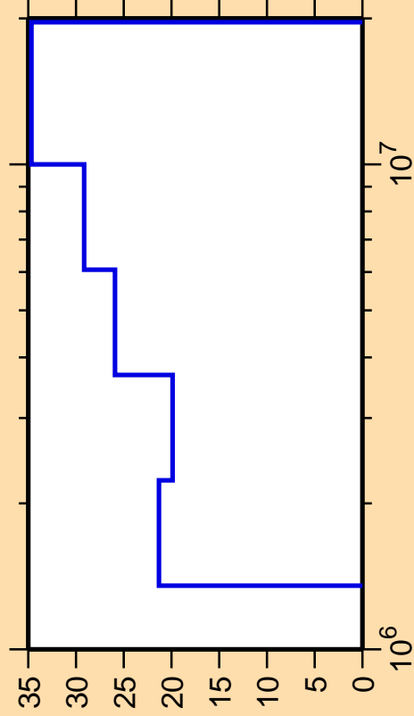
\Delta\sigma/\sigma vs. E for ^{42}\text{K}(n,\alpha)
