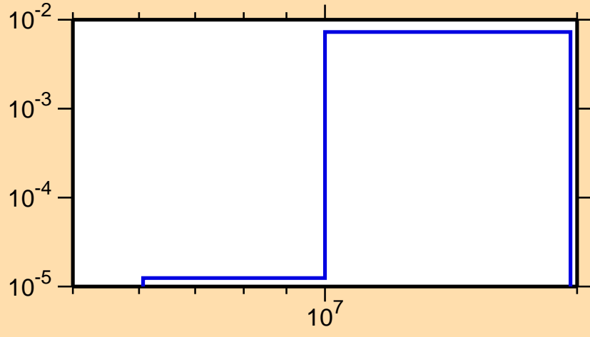
\sigma vs. E for ^{42}\text{K}(n,d)
