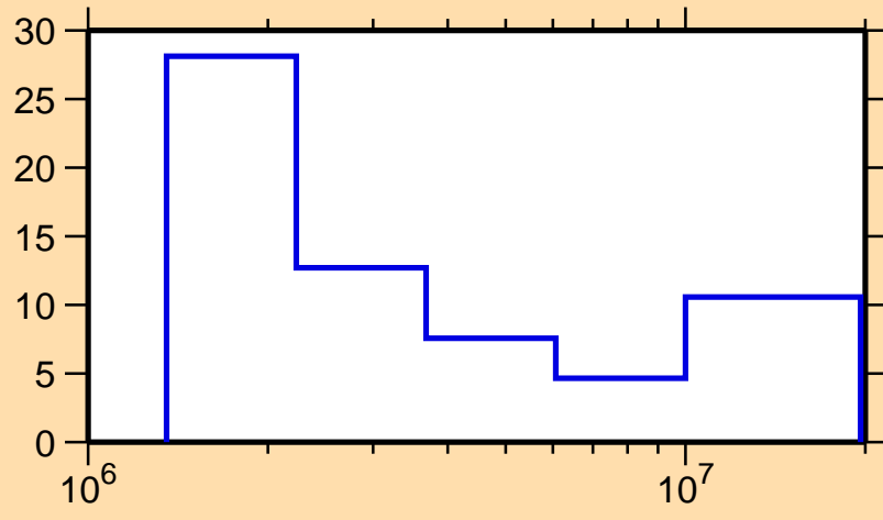
\Delta\sigma/\sigma vs. E for ^{42}\text{K}(n,n\text{cont.})
