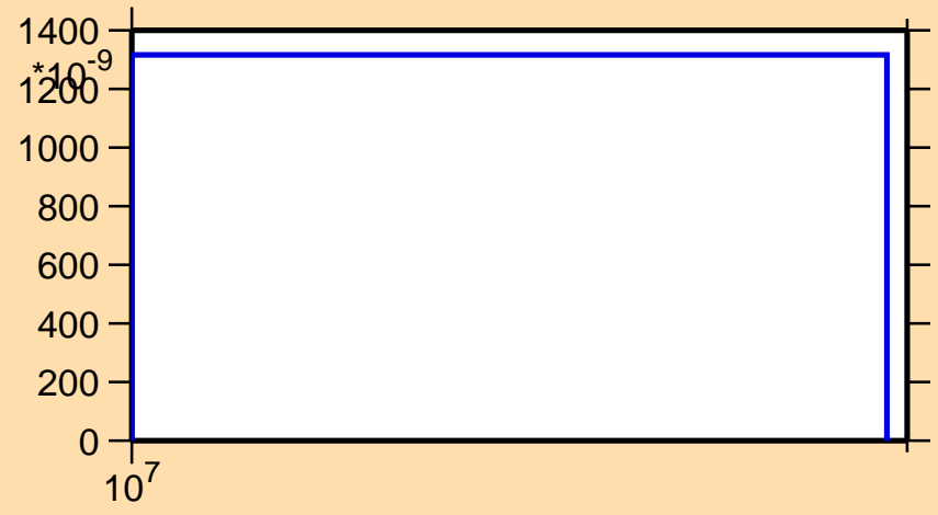
\sigma vs. E for ^{42}\text{K}(n,3n)
