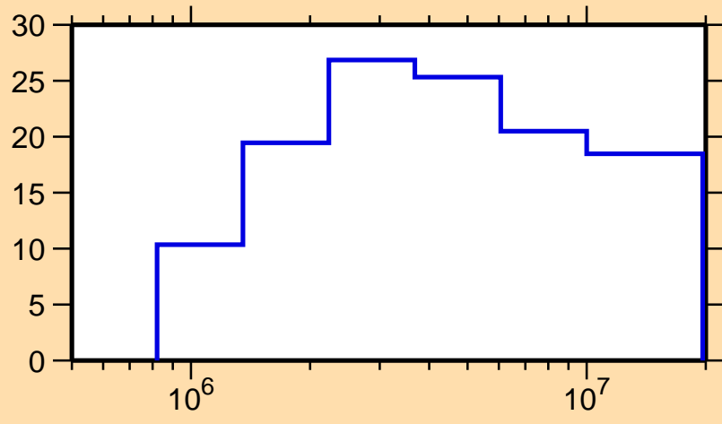
\Delta\sigma/\sigma vs. E for ^{42}\text{K}(n,p)
