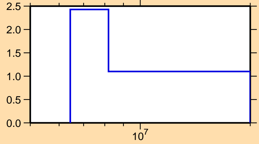
\Delta\sigma/\sigma vs. E for ^{42}\text{K}(n,\text{tot.})
