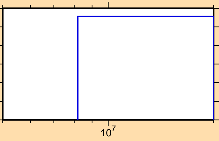
\sigma vs. E for ^{42}\text{K}(n,2np)
