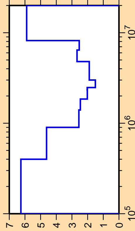
\Delta\sigma/\sigma vs. E for ^{42}\text{K}(n,\text{inel.})
