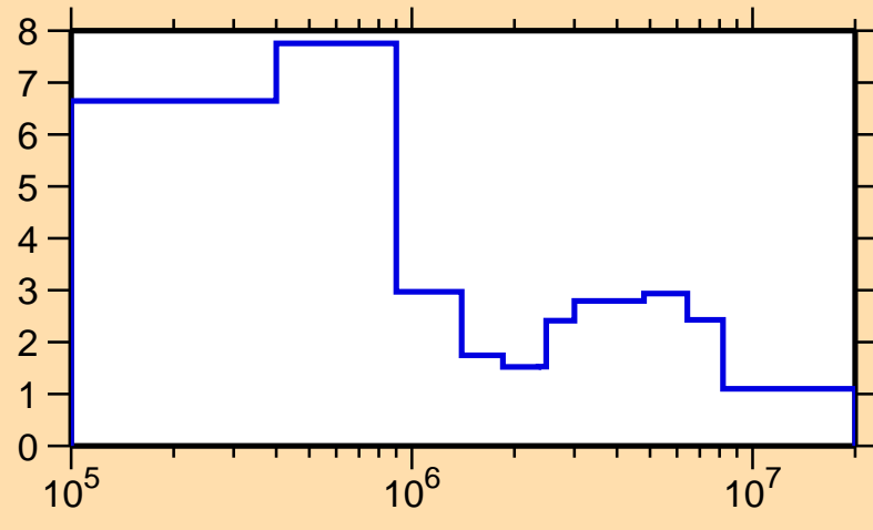
\Delta\sigma/\sigma vs. E for ^{42}\text{K}(n,\text{tot.})
