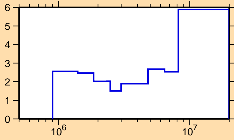
\Delta\sigma/\sigma vs. E for ^{42}\text{K}(n,\text{inel.})
