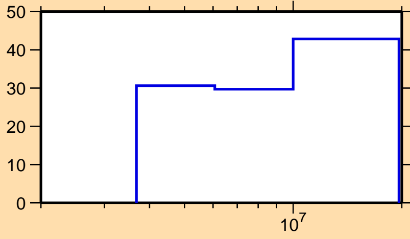
\Delta\sigma/\sigma vs. E for ^{43}\text{K}(n,\gamma)
