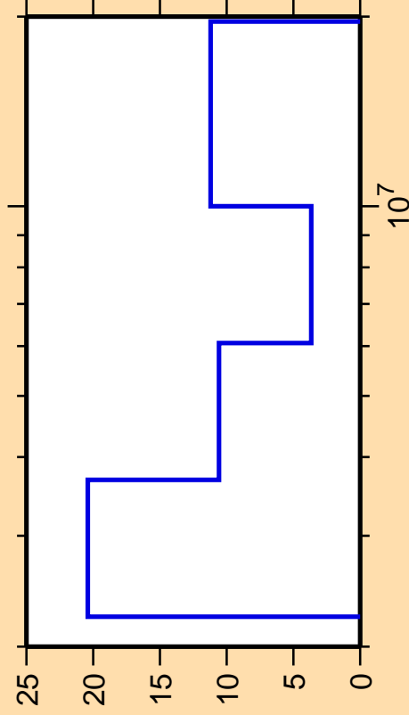
\Delta\sigma/\sigma vs. E for ^{43}\text{K}(n,ncont.)
