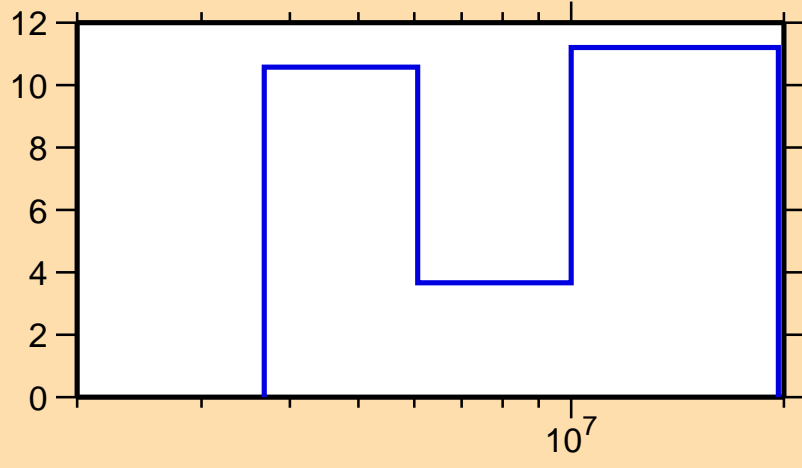
\Delta\sigma/\sigma vs. E for ^{43}\text{K}(n,n\text{cont.})
