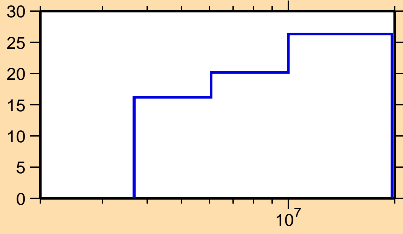
\Delta\sigma/\sigma vs. E for ^{43}\text{K}(n,p)
