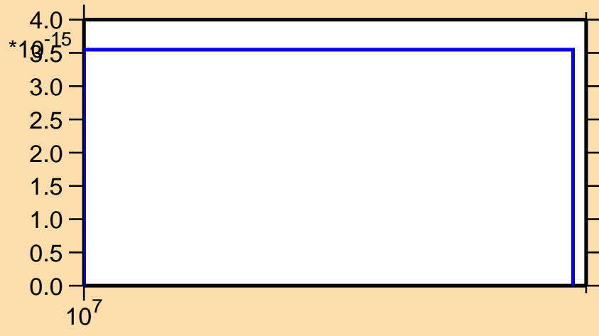
\sigma vs. E for ^{43}\text{K}(n,2n\alpha)
