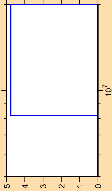
\Delta\sigma/\sigma vs. E for ^{43}\text{K}(n,2n)
