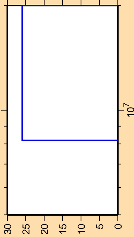
\Delta\sigma/\sigma vs. E for ^{43}\text{K}(n,p)
