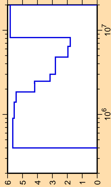
\Delta\sigma/\sigma vs. E for ^{43}\text{K}(n,\text{inel.})
