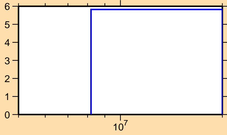
\Delta\sigma/\sigma vs. E for ^{43}\text{K}(n,\text{inel.})
