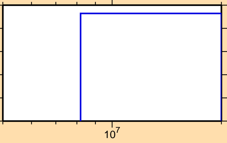
\sigma vs. E for ^{43}\text{K}(n,2np)
