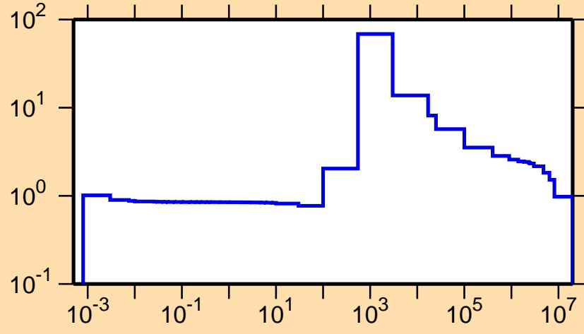
\sigma vs. E for ^{43}\text{K}(n,\text{el.})
