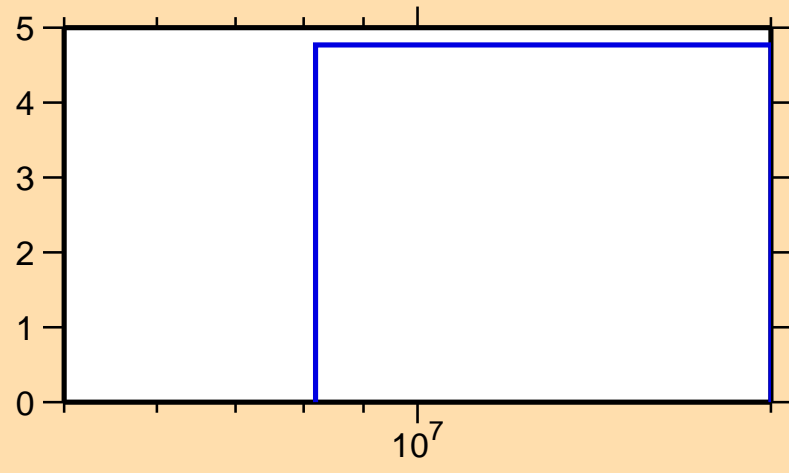
\Delta\sigma/\sigma vs. E for ^{43}\text{K}(n,2n)
