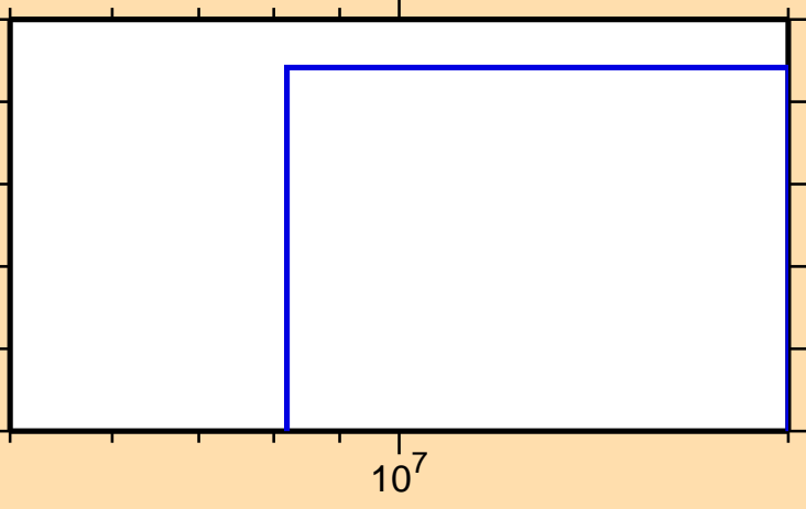
\sigma vs. E for ^{43}\text{K}(n,3n)
