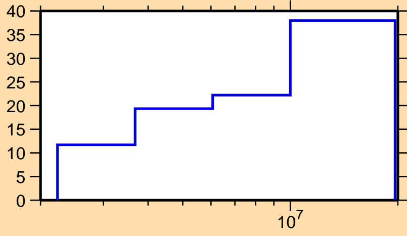
\Delta\sigma/\sigma vs. E for ^{44}\text{K}(n,n_1)
