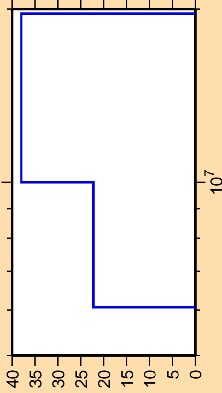
\Delta\sigma/\sigma vs. E for ^{44}\text{K}(n,n_1)
