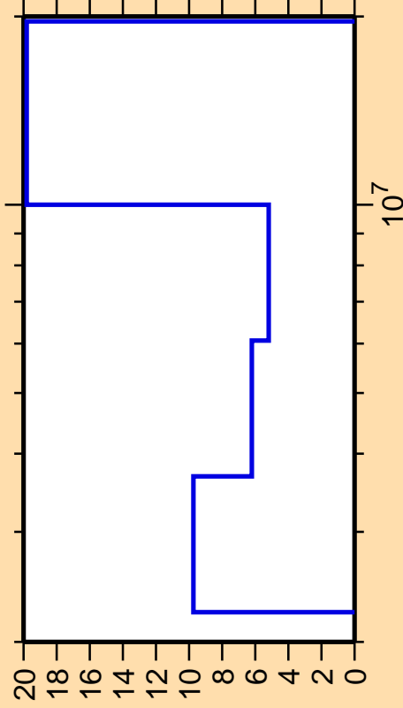
\Delta\sigma/\sigma vs. E for ^{44}\text{K}(n,ncont.)
