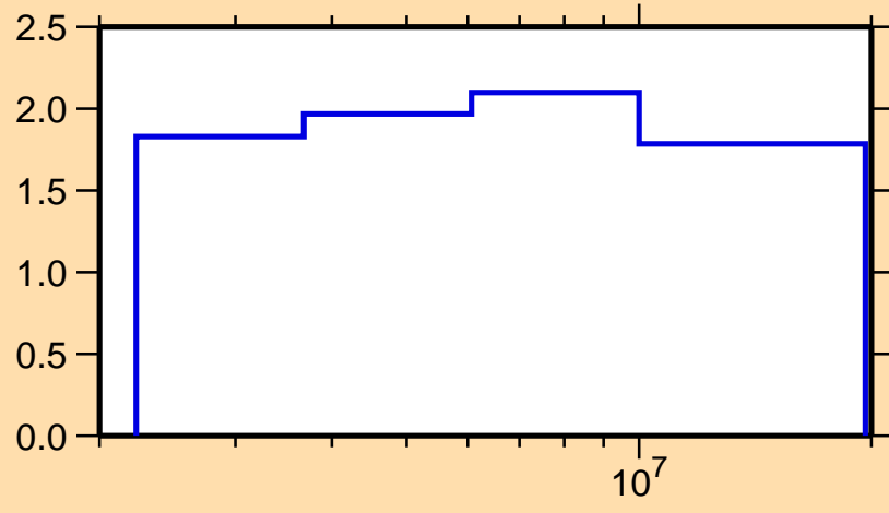
\Delta\sigma/\sigma vs. E for ^{44}\text{K}(n,tot.)
