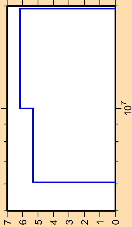
\Delta\sigma/\sigma vs. E for ^{44}\text{K}(n,2n)
