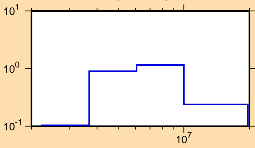
\sigma vs. E for ^{44}\text{K}(n,n\text{cont.})
