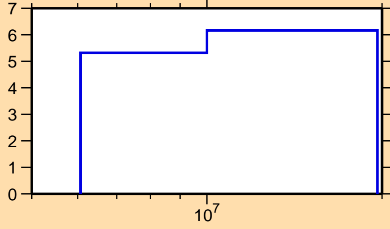
\Delta\sigma/\sigma vs. E for ^{44}\text{K}(n,2n)
