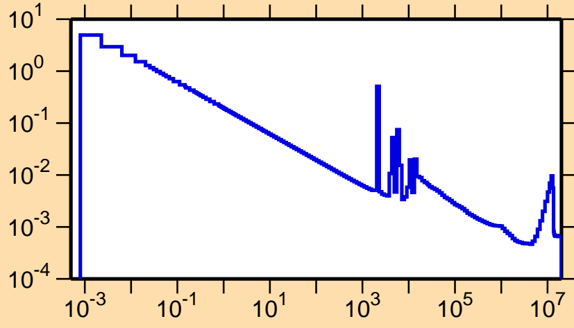
\sigma vs. E for ^{45}\text{K}(n,\gamma)
