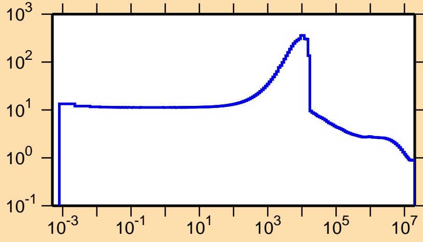
\sigma vs. E for ^{45}\text{K}(n,\text{el.})
