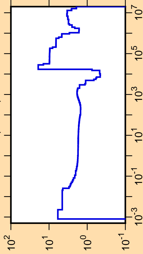
\Delta\sigma/\sigma vs. E for ^{45}\text{K}(n,\text{tot.})
