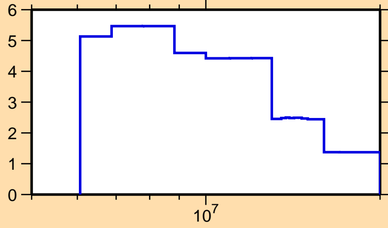
\Delta\sigma/\sigma vs. E for ^{45}\text{K}(n,el.)
