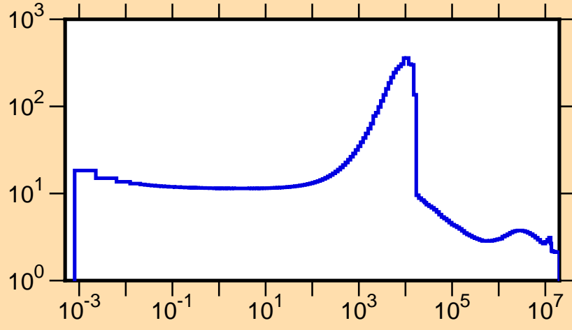
\sigma vs. E for ^{45}\text{K}(n,\text{tot.})
