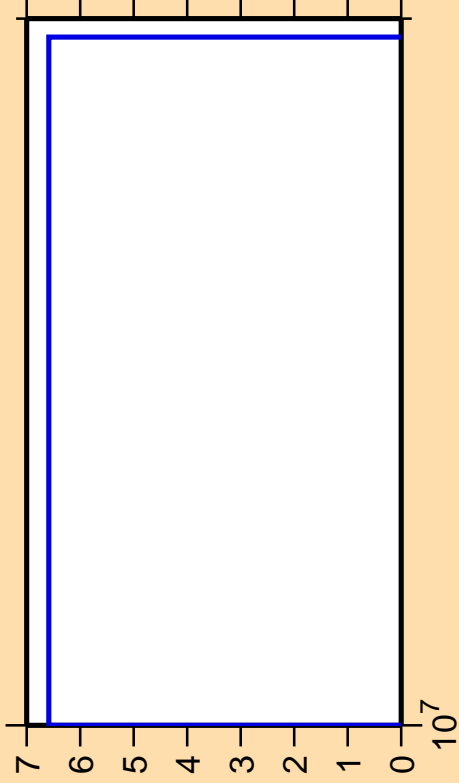
\Delta\sigma/\sigma vs. E for ^{45}\text{K}(n,3n)
