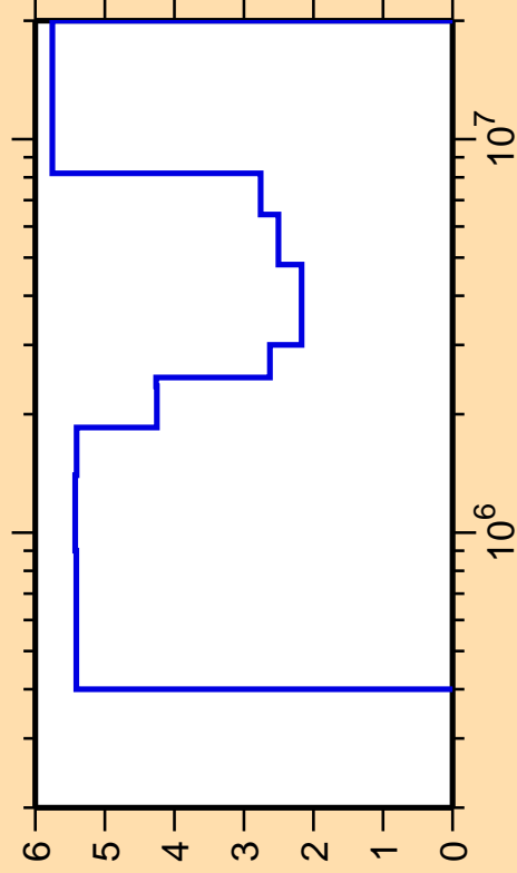
\Delta\sigma/\sigma vs. E for ^{45}\text{K}(n,\text{inel.})
