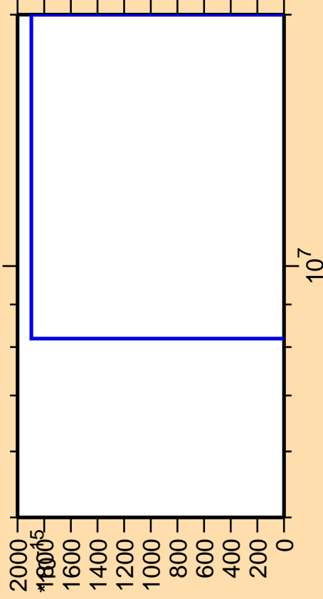
\Delta\sigma/\sigma vs. E for ^{45}\text{K}(n,\text{He}3)
