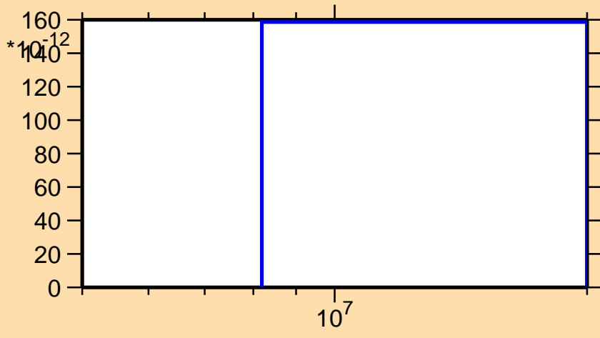
\sigma vs. E for ^{45}\text{K}(n,\text{nd})
