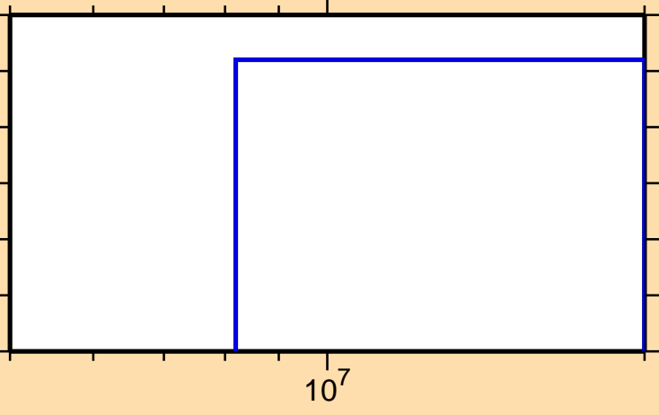
\sigma vs. E for ^{45}\text{K}(n,n\alpha)
