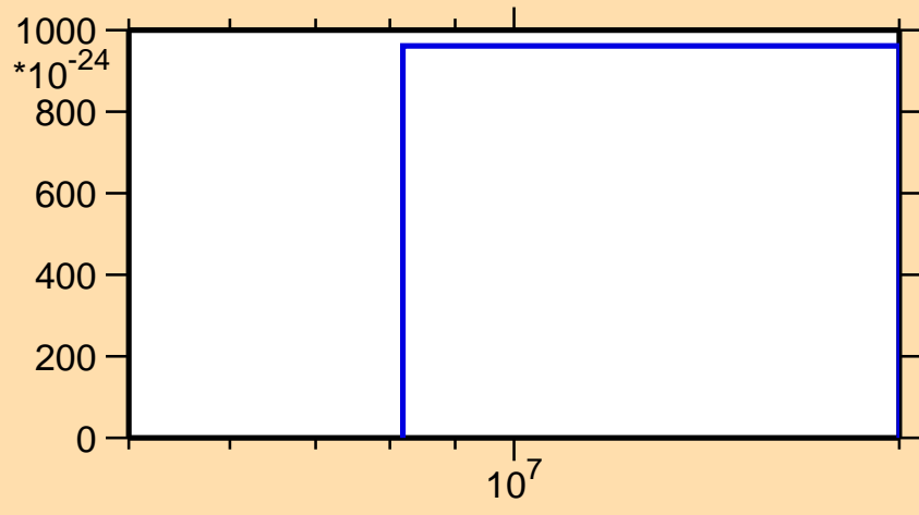
\sigma vs. E for ^{45}\text{K}(n,2n\alpha)
