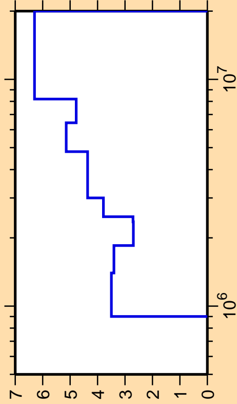
\Delta\sigma/\sigma vs. E for ^{45}\text{K}(n,n_3)
