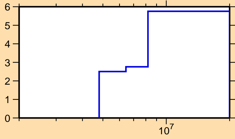
\Delta\sigma/\sigma vs. E for ^{45}\text{K}(n,\text{inel.})
