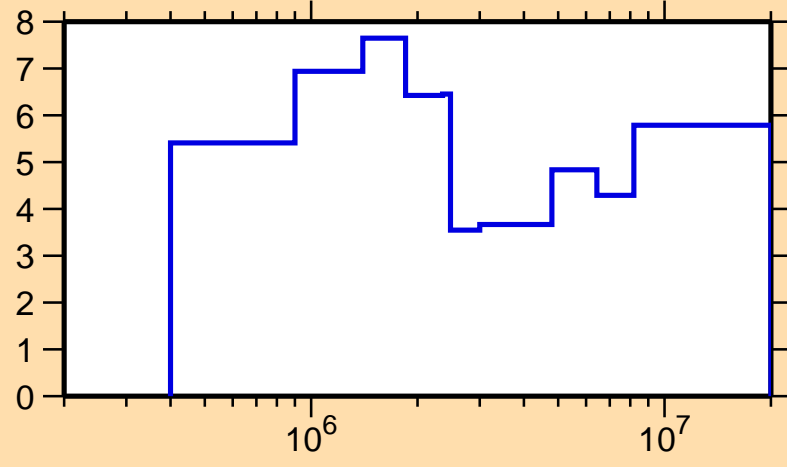
\Delta\sigma/\sigma vs. E for ^{45}\text{K}(n,n_1)
