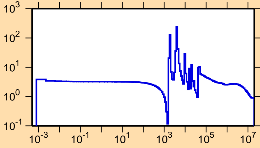
\sigma vs. E for ^{46}\text{K}(n,\text{el.})
