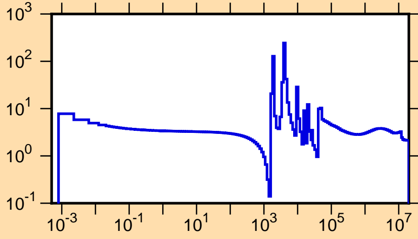
\sigma vs. E for ^{46}\text{K}(n,\text{tot.})
