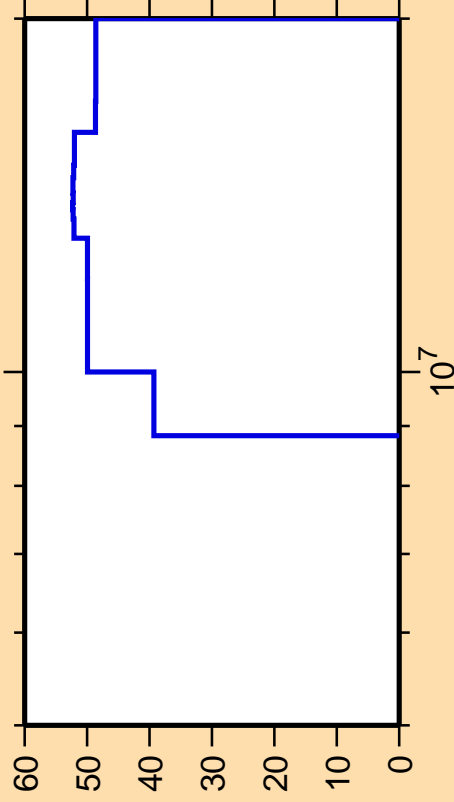
\Delta\sigma/\sigma vs. E for ^{46}\text{K}(n,n_1)
