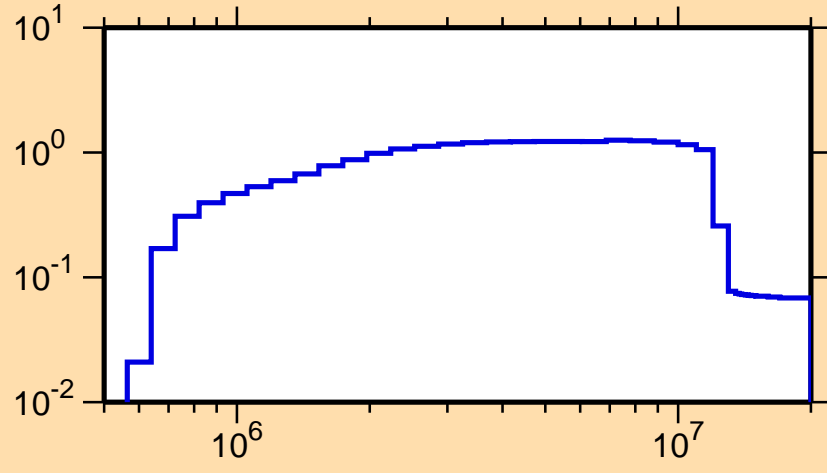
\sigma vs. E for ^{46}\text{K}(n,\text{inel.})
