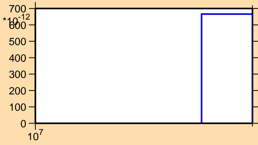
\sigma vs. E for ^{46}\text{K}(n,2np)
