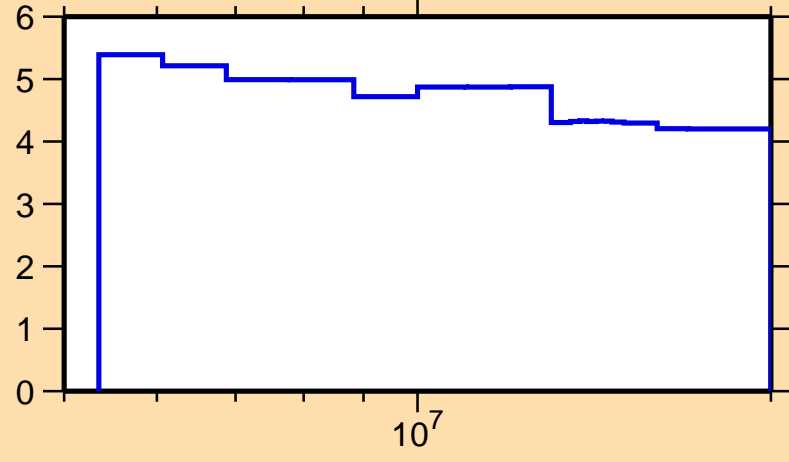
\Delta\sigma/\sigma vs. E for ^{46}\text{K}(n,\text{tot.})
