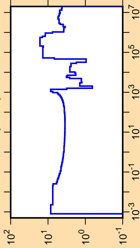
\Delta\sigma/\sigma vs. E for ^{46}\text{K}(n,\text{tot.})
