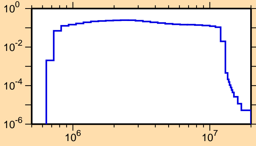
\sigma vs. E for ^{46}\text{K}(n,n_2)
