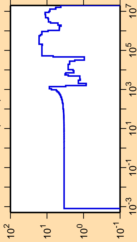
\Delta\sigma/\sigma vs. E for ^{46}\text{K}(n,\text{el.})
