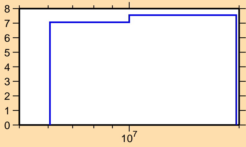
\Delta\sigma/\sigma vs. E for ^{46}\text{K}(n,\text{nonel.})
