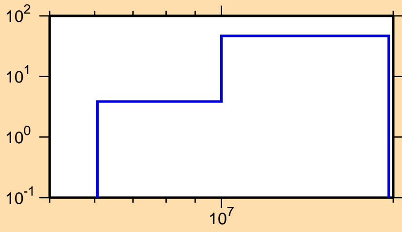
\Delta\sigma/\sigma vs. E for ^{46}\text{K}(n,inel.)
