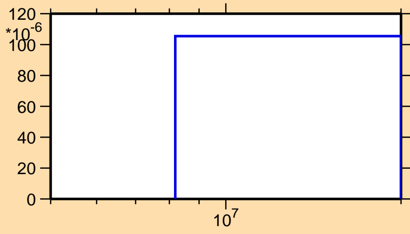
\sigma vs. E for ^{46}\text{K}(n,t)
