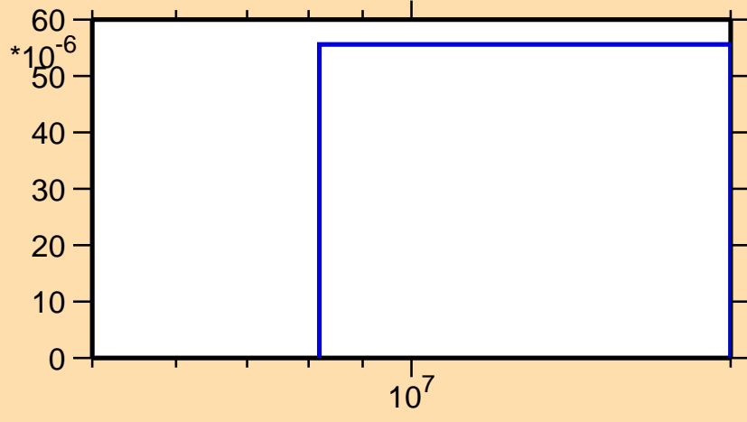
\sigma vs. E for ^{46}\text{K}(n,np)
