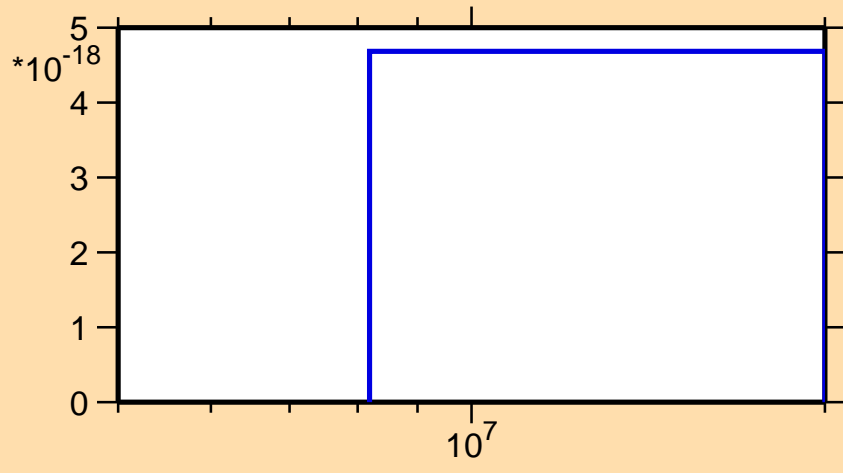
\sigma vs. E for ^{46}\text{K}(n,2n\alpha)
