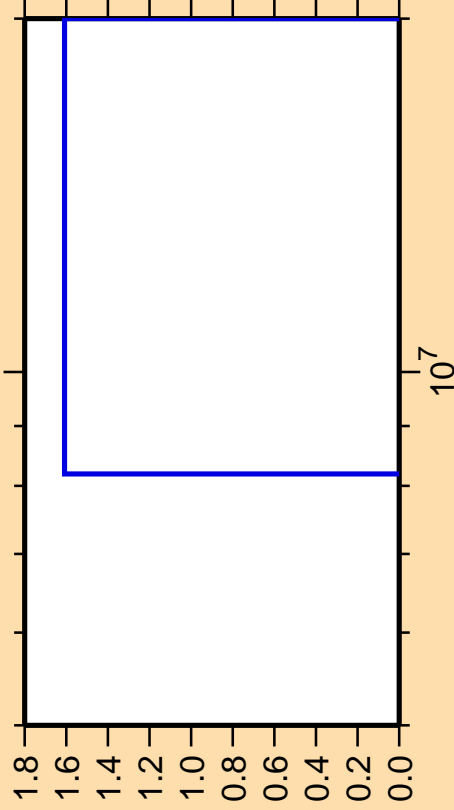
\Delta\sigma/\sigma vs. E for ^{46}\text{K}(n,nt)
