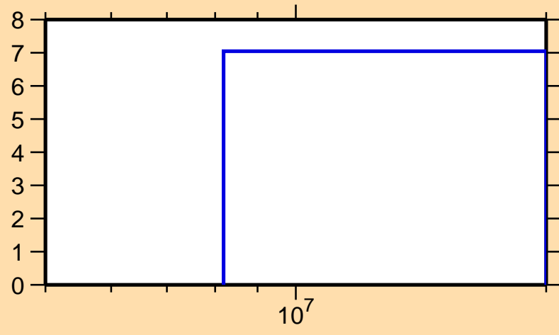
\Delta\sigma/\sigma vs. E for ^{46}\text{K}(n,\text{el.})
