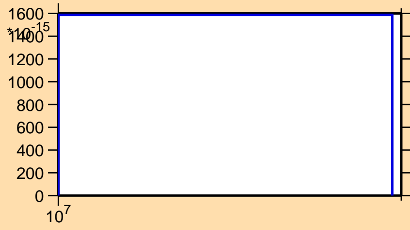
\sigma vs. E for ^{47}\text{K}(n,nt)
