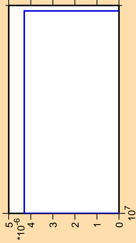
\Delta\sigma/\sigma vs. E for ^{47}\text{K}(n,nd)
