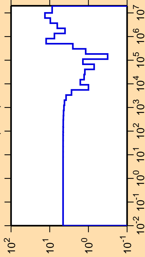
\Delta\sigma/\sigma vs. E for ^{47}\text{K}(n,\text{el.})
