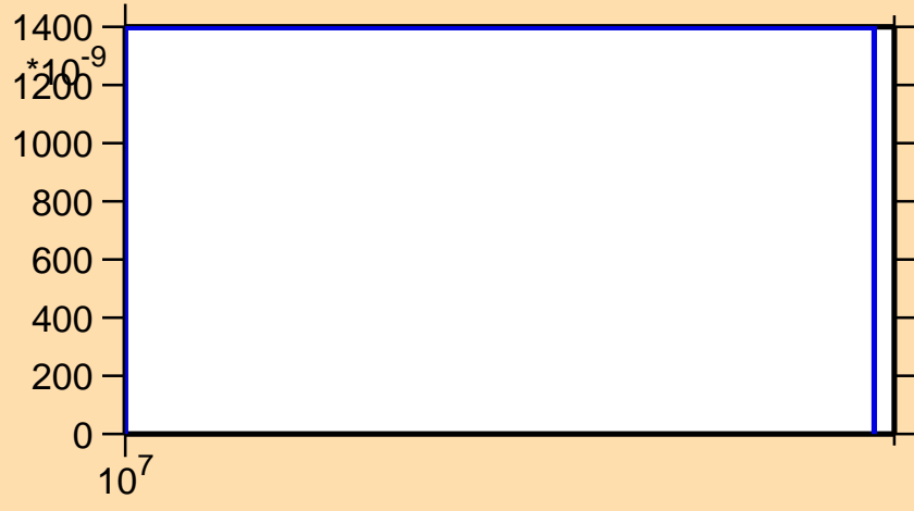
\sigma vs. E for ^{47}\text{K}(n,t)
