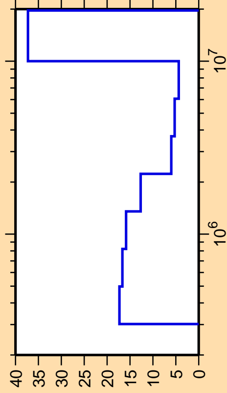
\Delta\sigma/\sigma vs. E for ^{47}\text{K}(n,\text{inel.})
