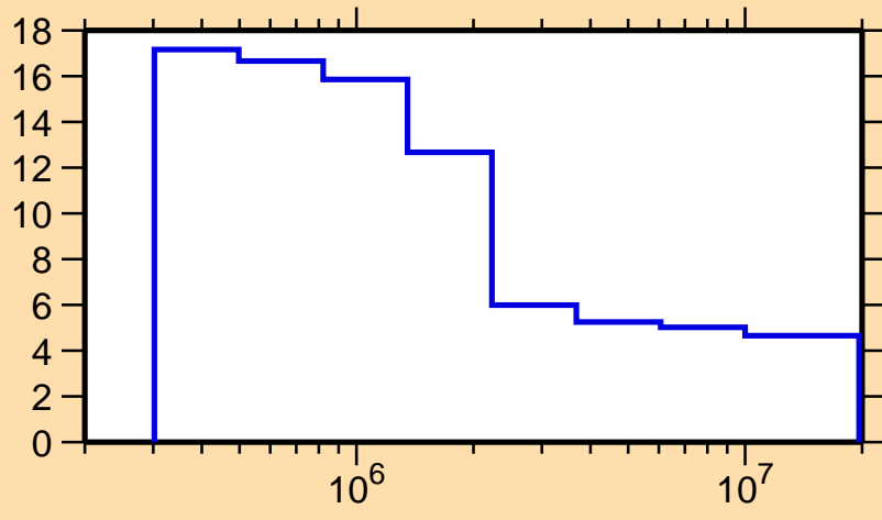
\Delta\sigma/\sigma vs. E for ^{47}\text{K}(n,\text{nonel.})
