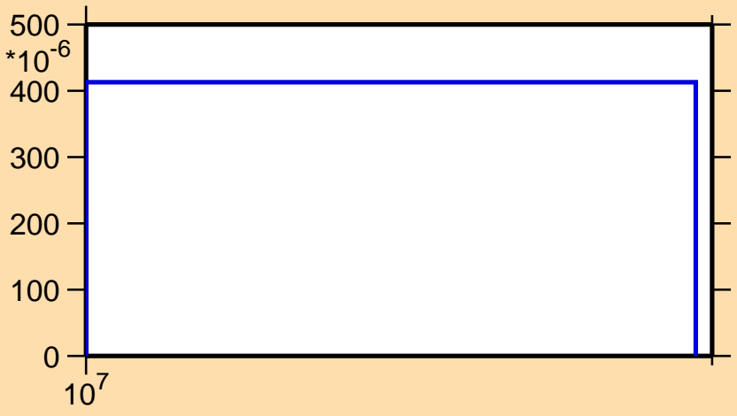
\sigma vs. E for ^{47}\text{K}(n,d)
