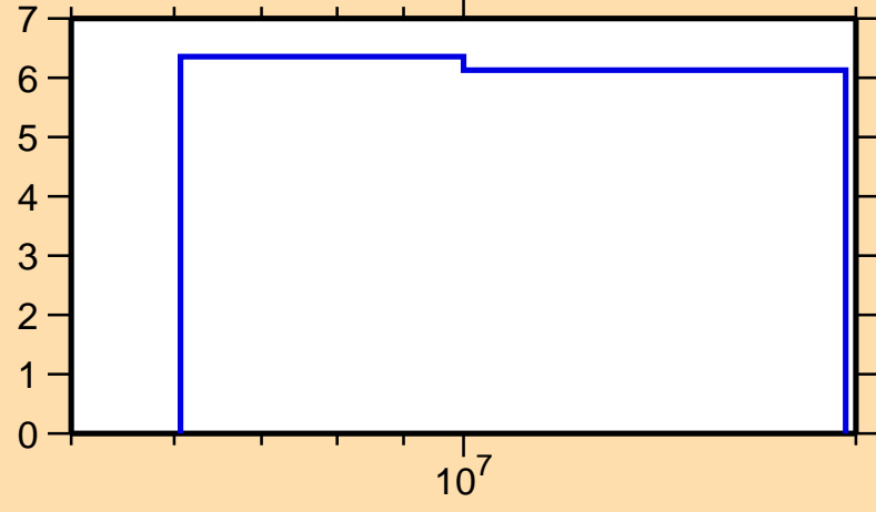
\Delta\sigma/\sigma vs. E for ^{47}\text{K}(n,2n)
