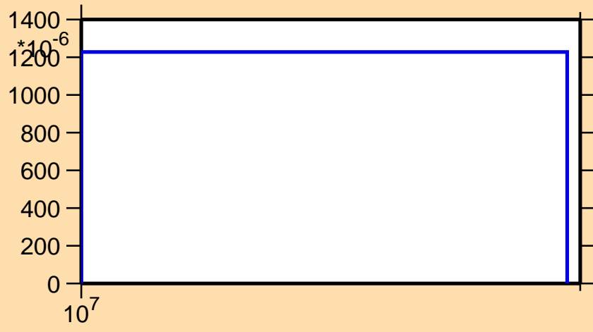
\sigma vs. E for ^{47}\text{K}(n,3n)
