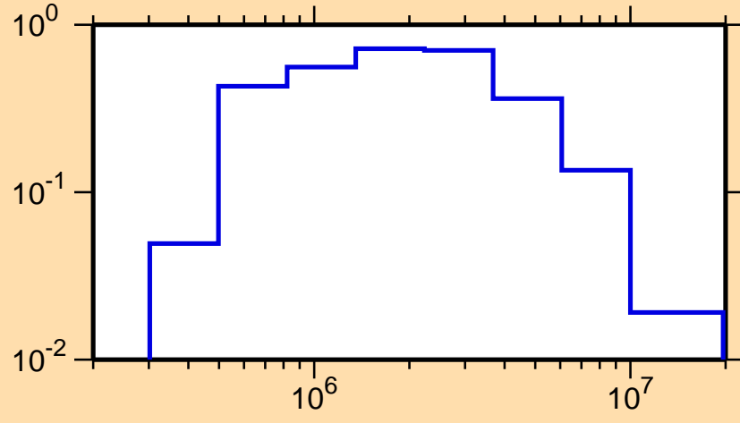
\sigma vs. E for ^{47}\text{K}(n,n_1)
