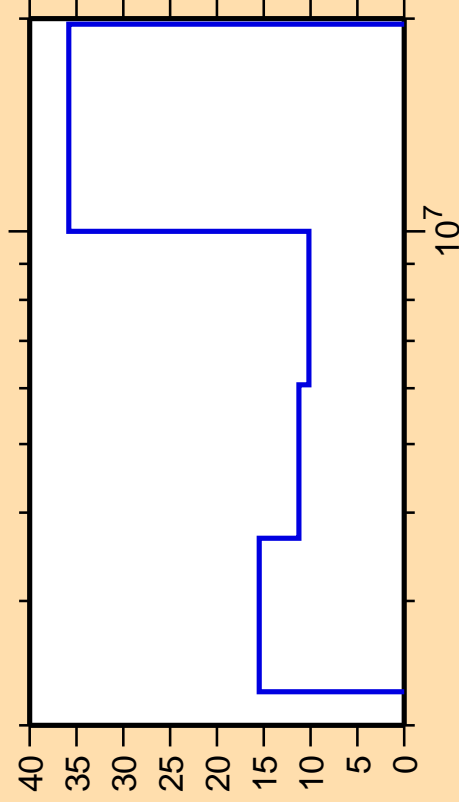
\Delta\sigma/\sigma vs. E for ^{47}\text{K}(n,n_4)
