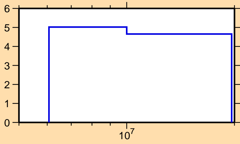
\Delta\sigma/\sigma vs. E for ^{47}\text{K}(n,\text{nonel.})
