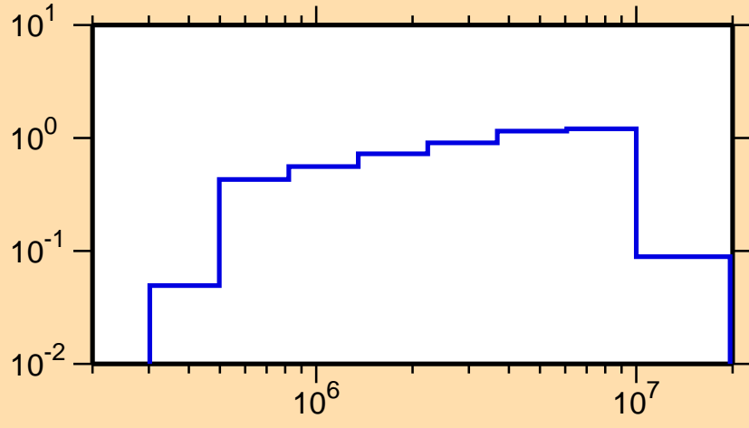
\sigma vs. E for ^{47}\text{K}(n,\text{inel.})
