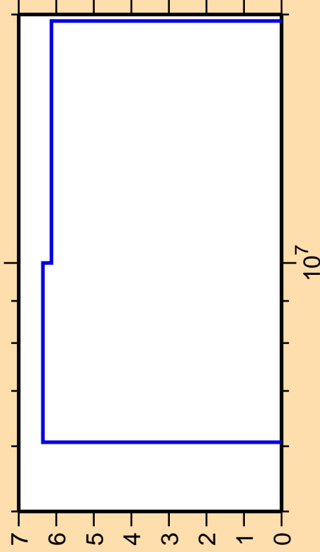
\Delta\sigma/\sigma vs. E for ^{47}\text{K}(n,2n)
