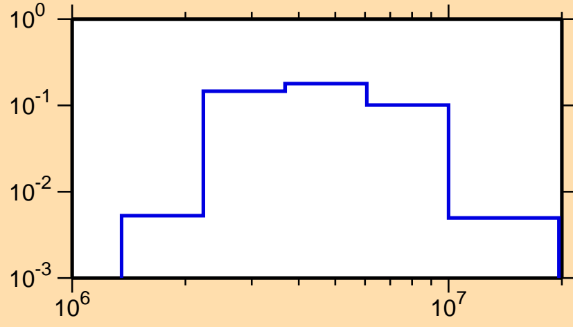
\sigma vs. E for ^{47}\text{K}(n,n_2)
