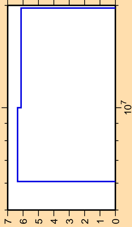
\Delta\sigma/\sigma vs. E for ^{47}\text{K}(n,2n)
