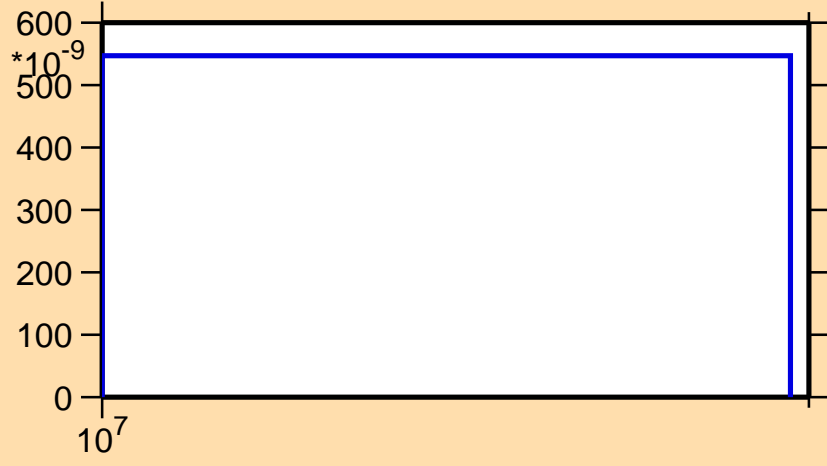
\sigma vs. E for ^{47}\text{K}(n,np)
