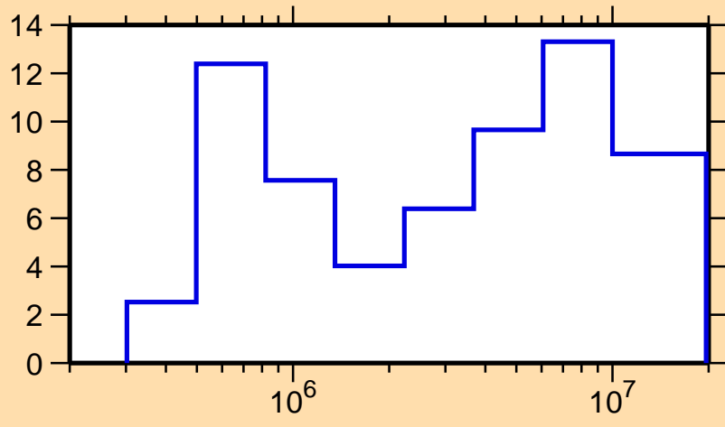
\Delta\sigma/\sigma vs. E for ^{47}\text{K}(n,\text{el.})
