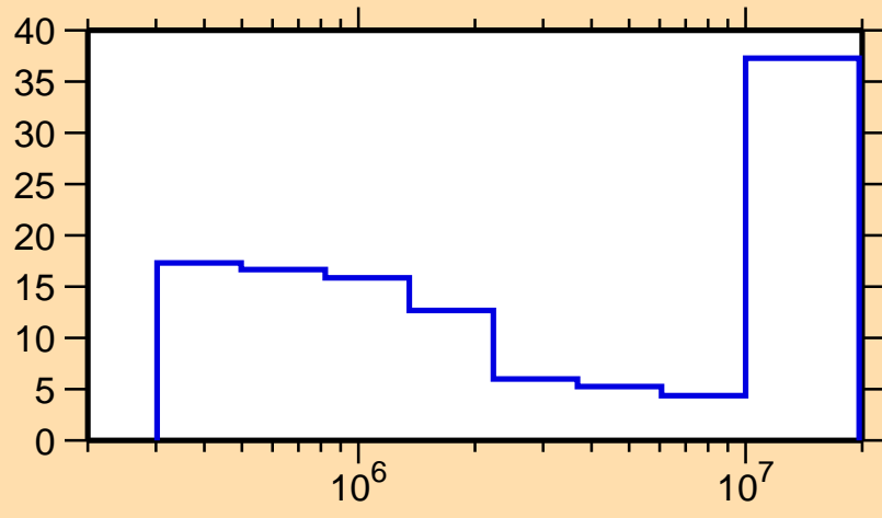
\Delta\sigma/\sigma vs. E for ^{47}\text{K}(n,\text{inel.})
