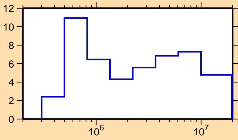
\Delta\sigma/\sigma vs. E for ^{47}\text{K}(n,\text{tot.})
