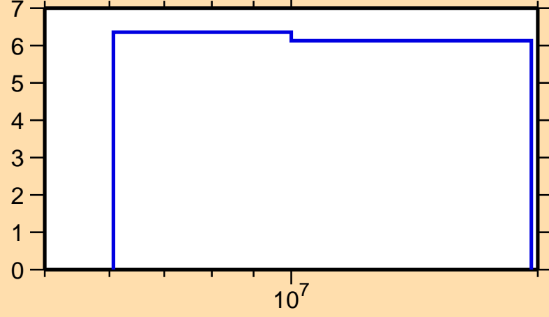
\Delta\sigma/\sigma vs. E for ^{47}\text{K}(n,2n)
