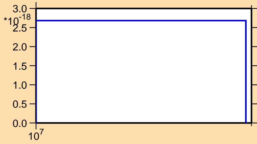
\sigma vs. E for ^{47}\text{K}(n,nd)
