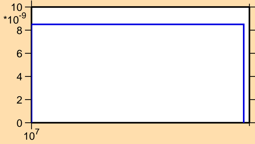
\sigma vs. E for ^{47}\text{K}(n,n\alpha)
