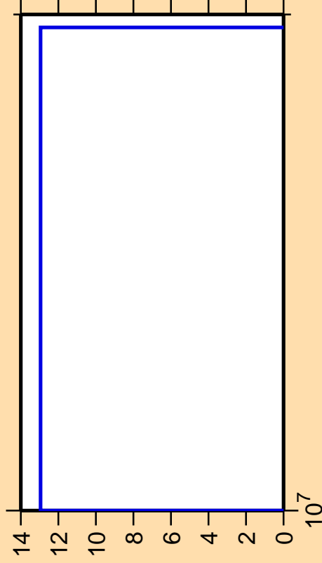
\Delta\sigma/\sigma vs. E for ^{47}\text{K}(n,3n)
