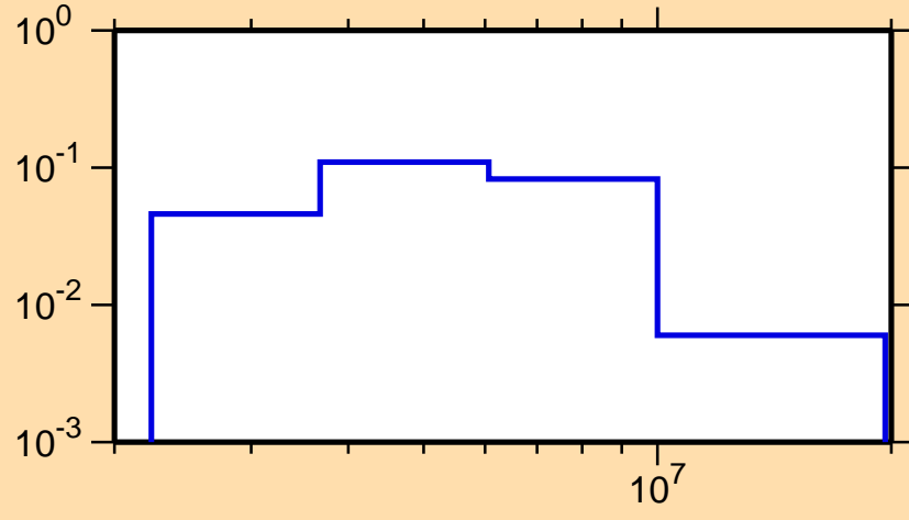
\sigma vs. E for ^{47}\text{K}(n,n_3)
