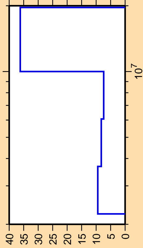
\Delta\sigma/\sigma vs. E for ^{47}\text{K}(n,n_3)
