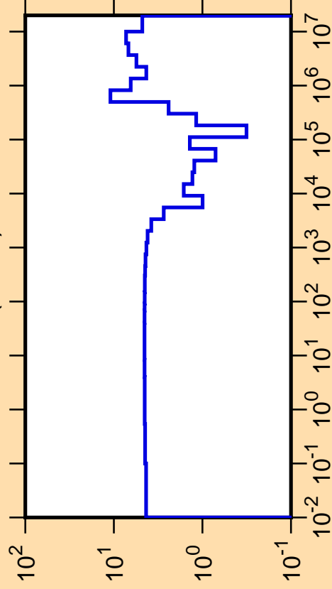
\Delta\sigma/\sigma vs. E for ^{47}\text{K}(n,\text{tot.})
