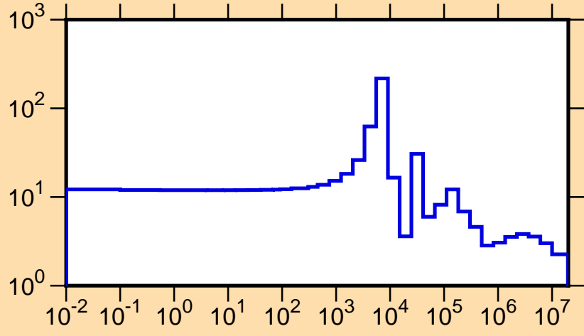
\sigma vs. E for ^{47}\text{K}(n,\text{tot.})
