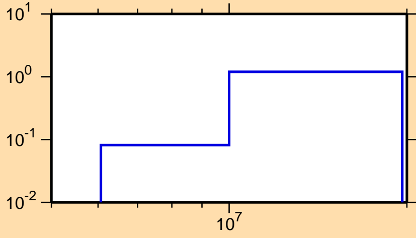
\sigma vs. E for ^{47}\text{K}(n,2n)
