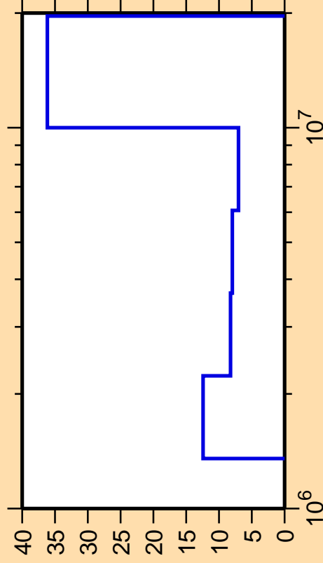
\Delta\sigma/\sigma vs. E for ^{47}\text{K}(n,n_2)
