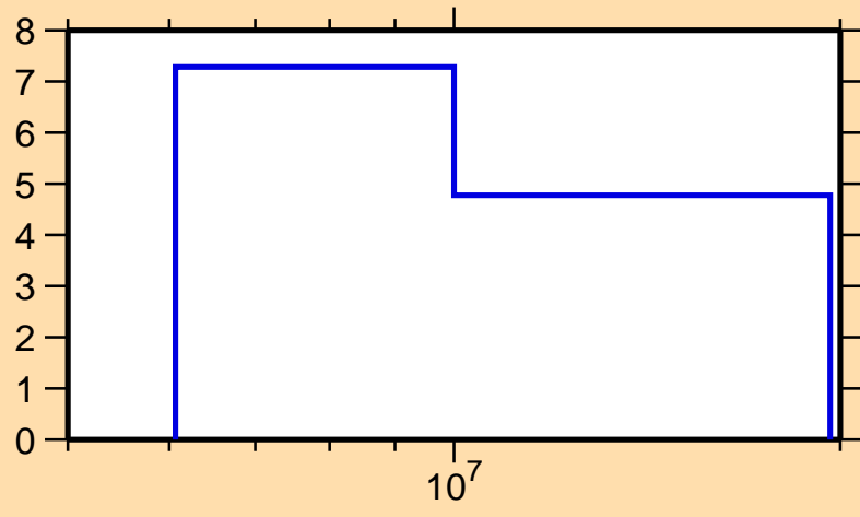
\Delta\sigma/\sigma vs. E for ^{47}\text{K}(n,\text{tot.})
