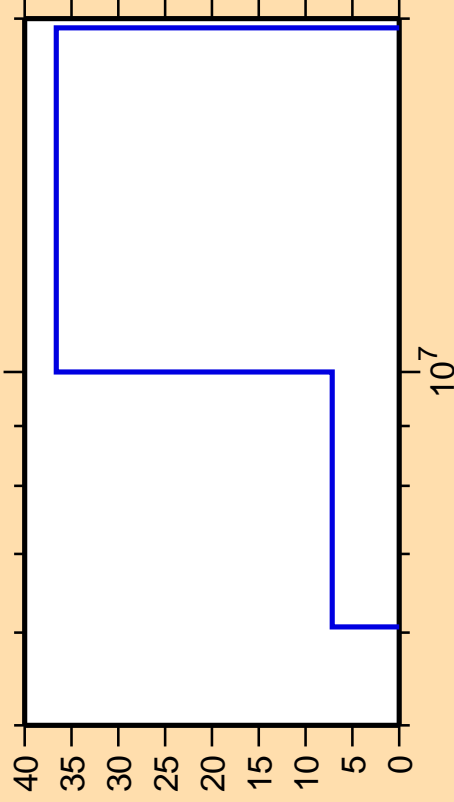
\Delta\sigma/\sigma vs. E for ^{47}\text{K}(n,n_1)
