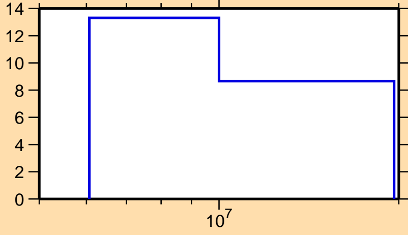
\Delta\sigma/\sigma vs. E for ^{47}\text{K}(n,\text{el.})
