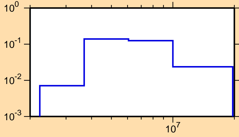
\sigma vs. E for ^{47}\text{K}(n,n_4)
