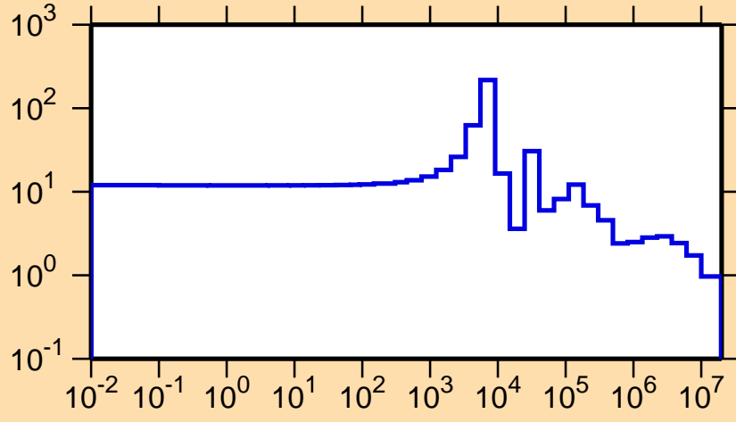
\sigma vs. E for ^{47}\text{K}(n,\text{el.})
