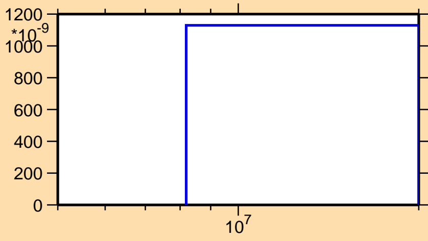
\sigma vs. E for ^{47}\text{K}(n,t)
