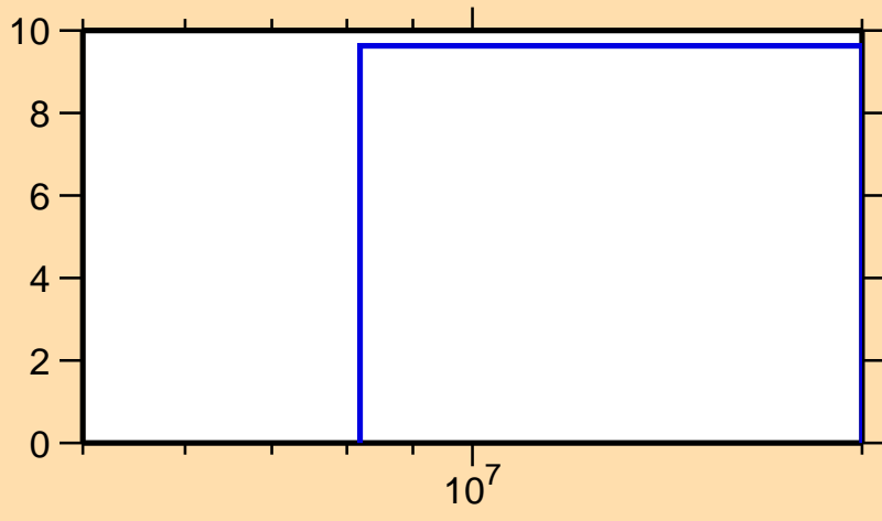
\Delta\sigma/\sigma vs. E for ^{47}\text{K}(n,el.)
