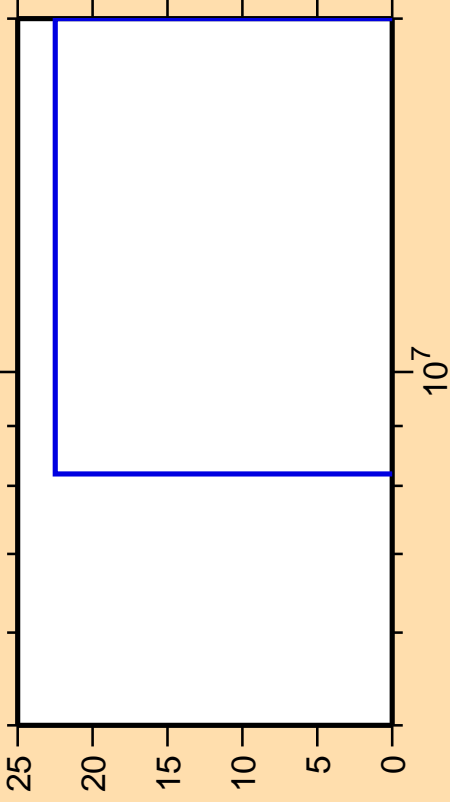
\Delta\sigma/\sigma vs. E for ^{47}\text{K}(n,p)
