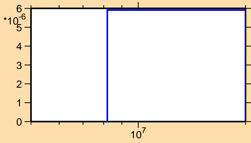
\sigma vs. E for ^{47}\text{K}(n,\alpha)
