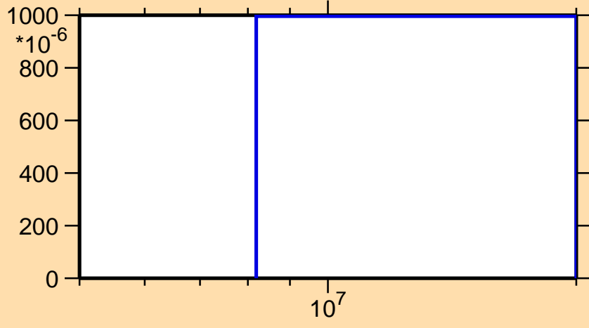
\sigma vs. E for ^{47}\text{K}(n,3n)
