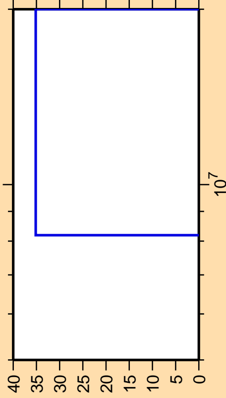
\Delta\sigma/\sigma vs. E for ^{47}\text{K}(n,\gamma)
