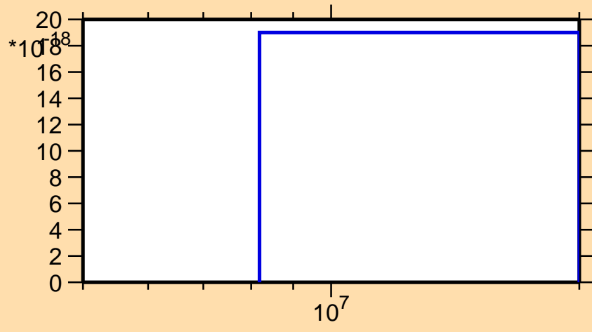
\sigma vs. E for ^{47}\text{K}(n,nd)
