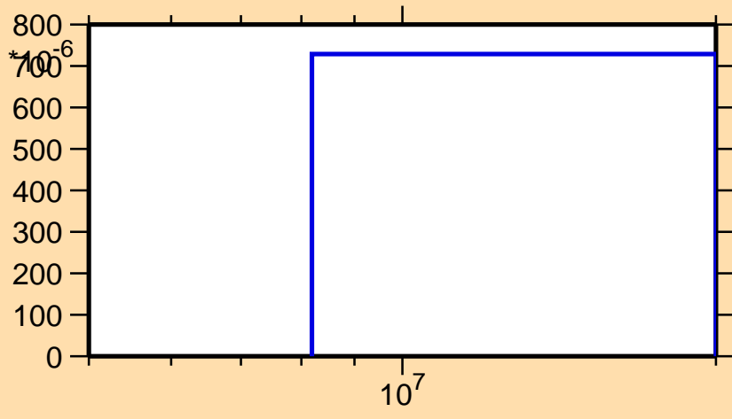
\sigma vs. E for ^{47}\text{K}(n,p)
