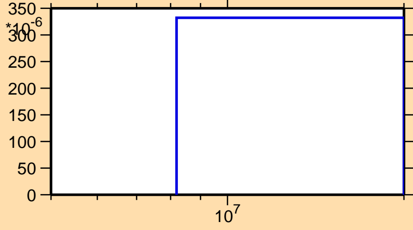
\sigma vs. E for ^{47}\text{K}(n,d)
