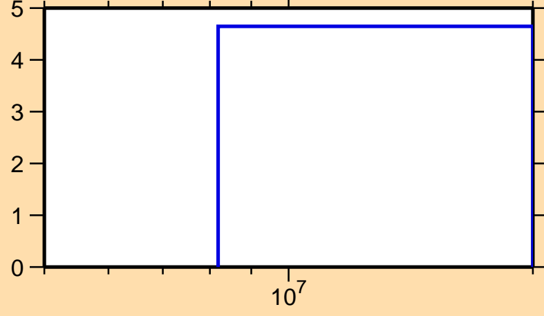
\Delta\sigma/\sigma vs. E for ^{47}\text{K}(n,\text{nonel.})
