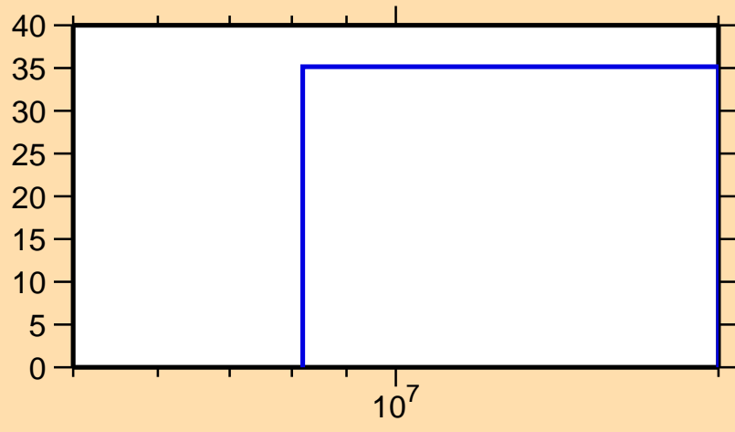
\Delta\sigma/\sigma vs. E for ^{47}\text{K}(n,\gamma)
