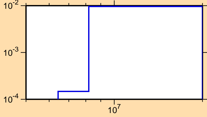
\sigma vs. E for ^{47}\text{K}(n,n\text{cont.})
