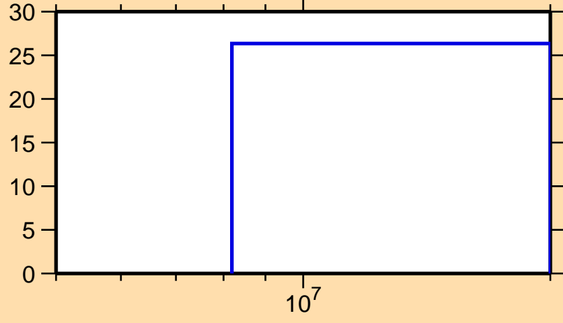
\Delta\sigma/\sigma vs. E for ^{47}\text{K}(n,n_1)
