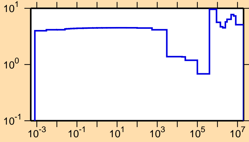
\Delta\sigma/\sigma vs. E for ^{47}\text{K}(n,\text{tot.})
