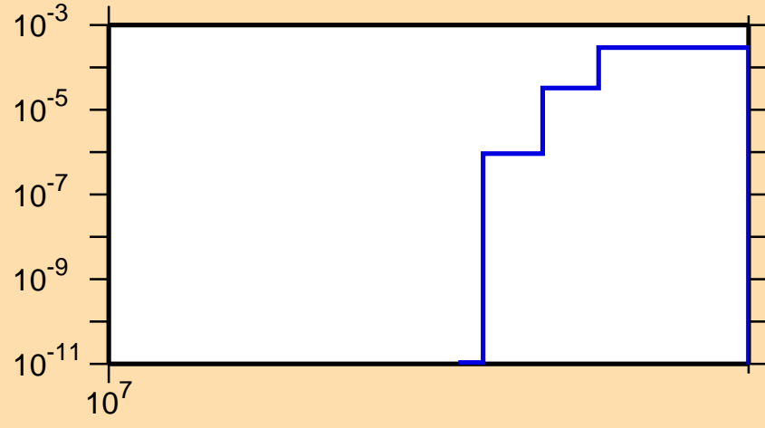
\sigma vs. E for ^{48}\text{K}(n,np)
