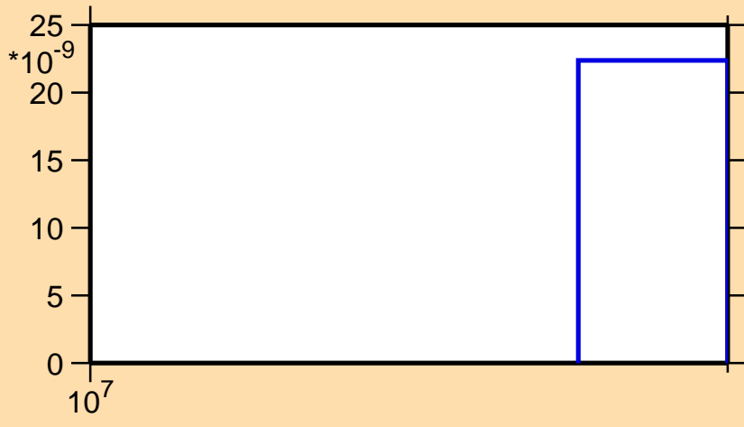
\sigma vs. E for ^{48}\text{K}(n,nt)
