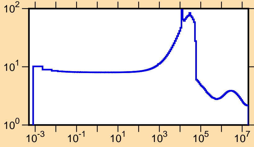
\sigma vs. E for ^{48}\text{K}(n,\text{tot.})
