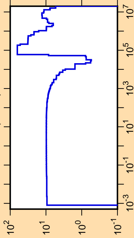
\Delta\sigma/\sigma vs. E for ^{48}\text{K}(n,\text{tot.})
