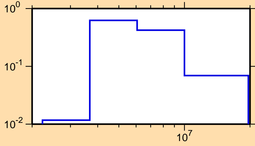
\sigma vs. E for ^{48}\text{K}(n,n\text{cont.})
