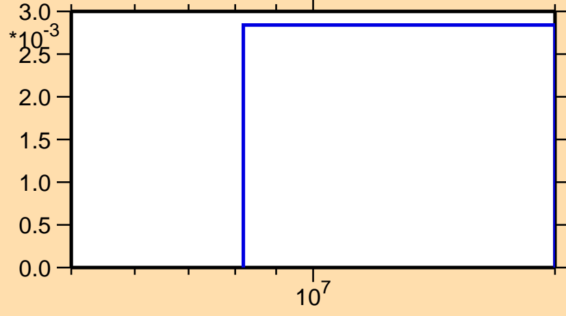
\sigma vs. E for ^{48}\text{K}(n,p)
