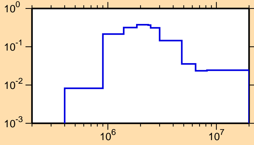
\sigma vs. E for ^{48}\text{K}(n,n_3)
