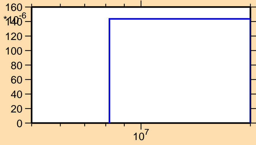
\sigma vs. E for ^{48}\text{K}(n,t)
