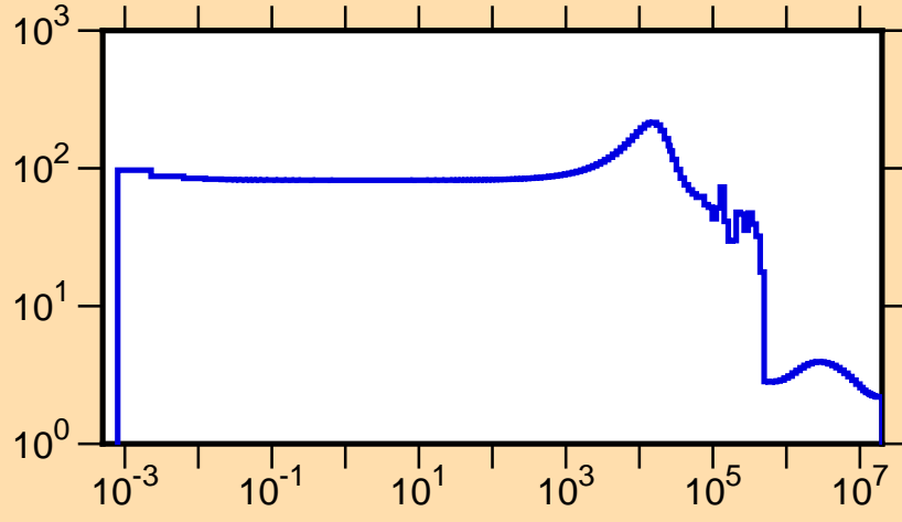
\sigma vs. E for ^{49}\text{K}(n,\text{tot.})
