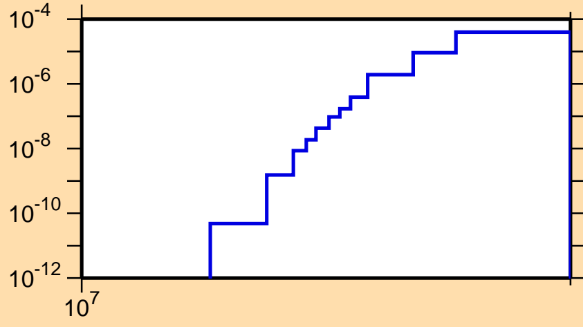
\sigma vs. E for ^{49}\text{K}(n,\alpha)
