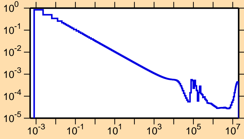
\sigma vs. E for ^{49}\text{K}(n,\gamma)
