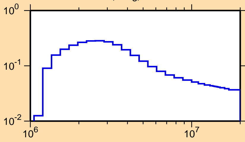
\sigma vs. E for ^{49}\text{K}(n,n_3)
