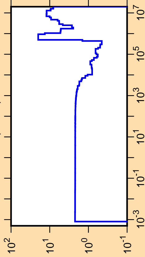
\Delta\sigma/\sigma vs. E for ^{49}\text{K}(n,\text{tot.})
