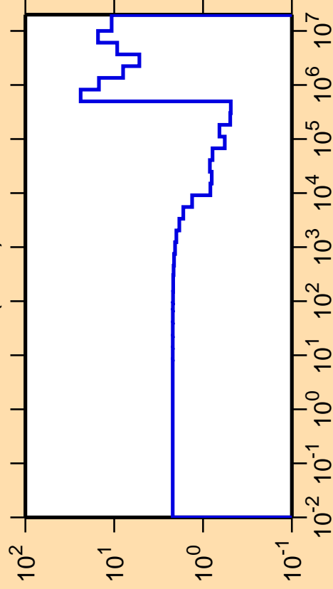
\Delta\sigma/\sigma vs. E for ^{49}\text{K}(n,\text{el.})
