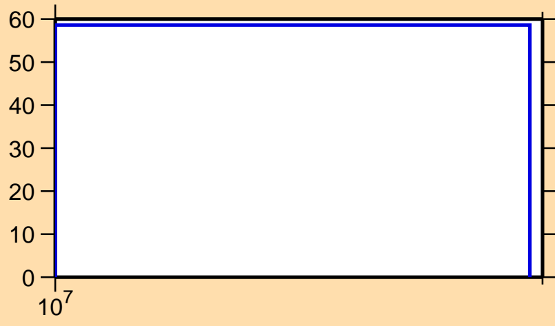
\Delta\sigma/\sigma vs. E for ^{49}\text{K}(n,p)
