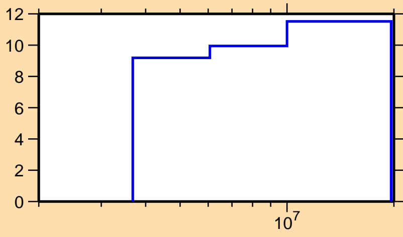
\Delta\sigma/\sigma vs. E for ^{49}\text{K}(n,n\text{onel.})
