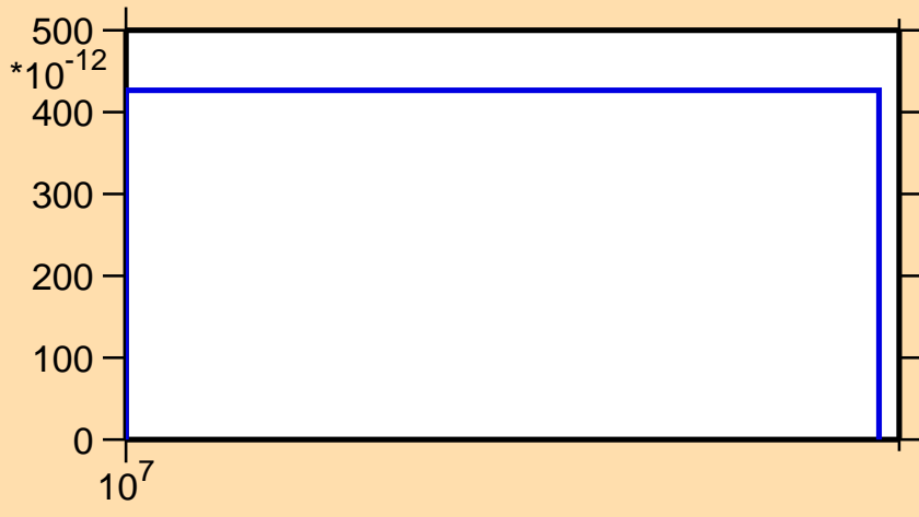
\sigma vs. E for ^{49}\text{K}(n,nd)
