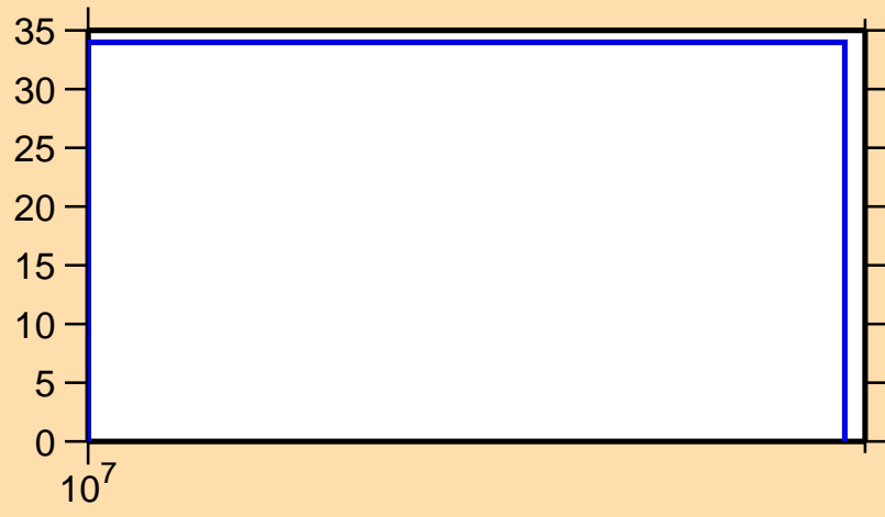
\Delta\sigma/\sigma vs. E for ^{49}\text{K}(n,ncont.)
