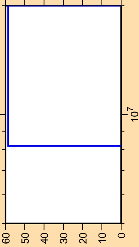
\Delta\sigma/\sigma vs. E for ^{49}\text{K}(n,p)
