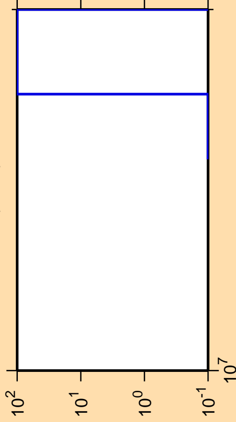
\Delta\sigma/\sigma vs. E for ^{72}\text{Kr}(n,\text{nd})
