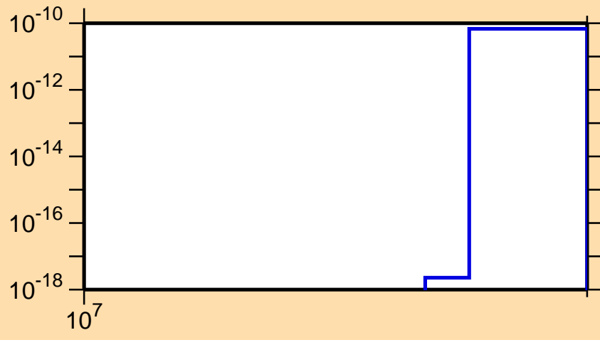
\sigma vs. E for ^{72}\text{Kr}(n,\text{nd})
