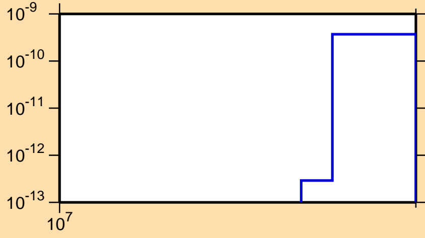
\sigma vs. E for ^{72}\text{Kr} (mt 34)
