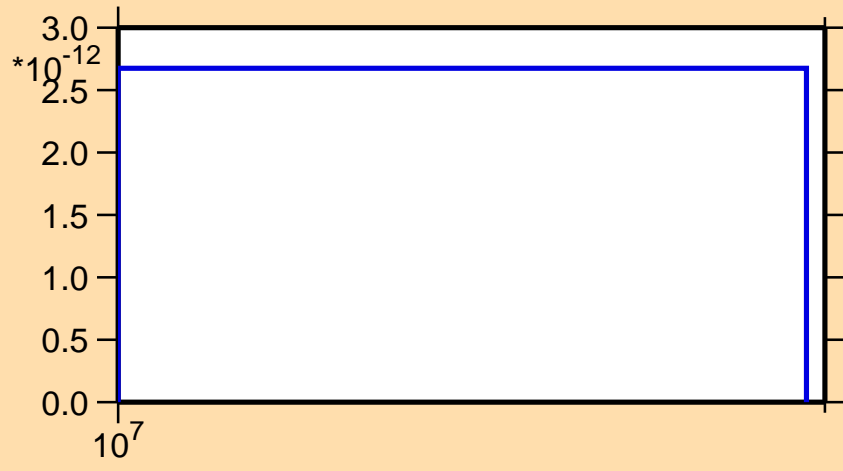
\sigma vs. E for ^{72}\text{Kr} (mt 34)
