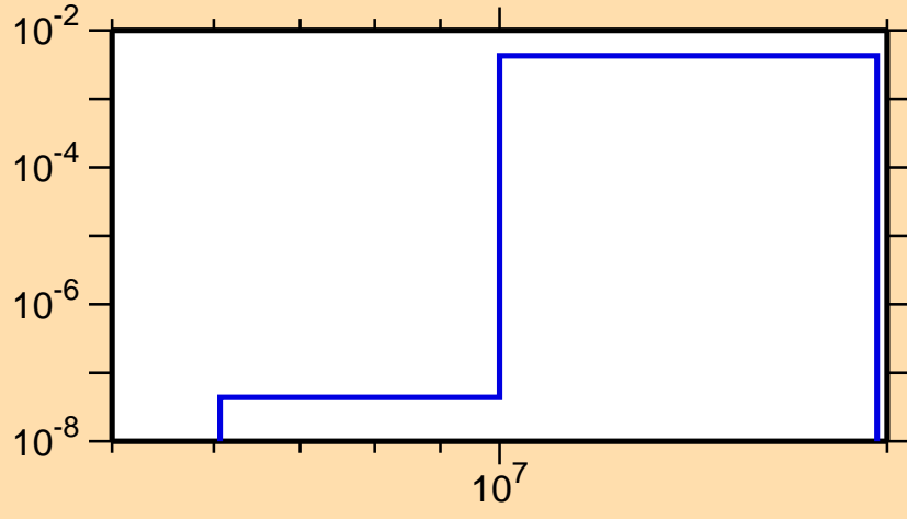
\sigma vs. E for ^{72}\text{Kr}(n,\text{pd})
