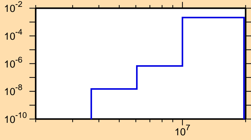
\sigma vs. E for ^{72}\text{Kr}(n,\text{He}3)
