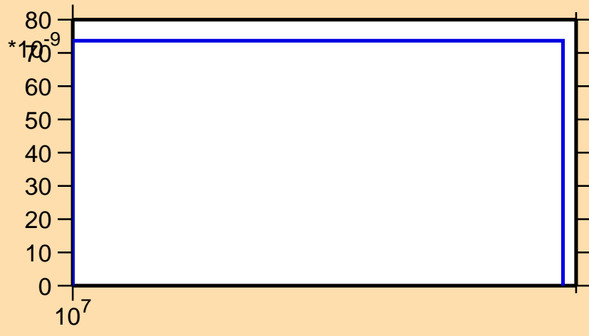
\sigma vs. E for ^{72}\text{Kr}(\text{mt } 45)
