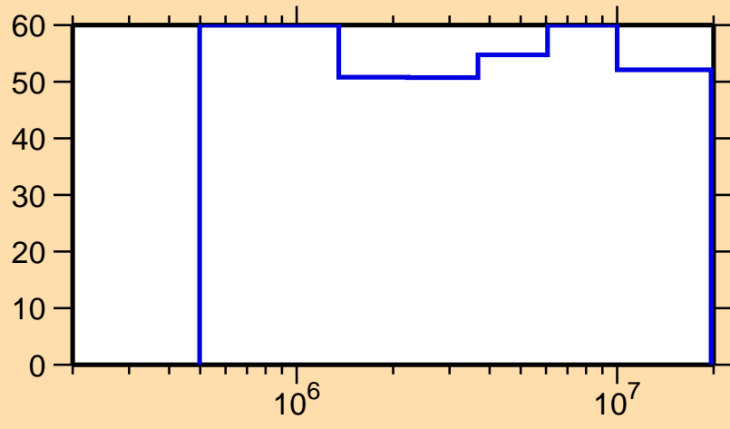
\Delta\sigma/\sigma vs. E for ^{72}\text{Kr}(n,n_1)
