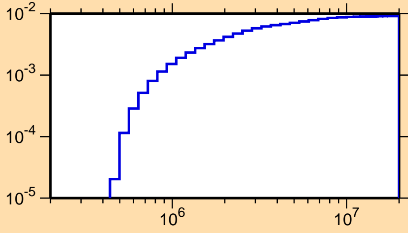
\sigma vs. E for ^{73}\text{Kr}(n,n_4)
