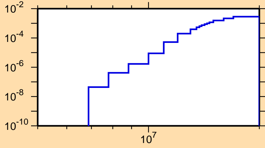
\sigma vs. E for ^{73}\text{Kr}(n,n\alpha)
