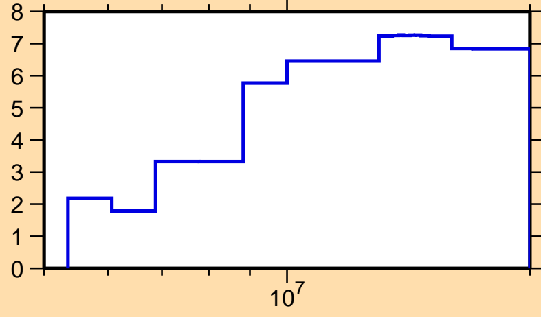
\Delta\sigma/\sigma vs. E for ^{73}\text{Kr}(n, tot.)
