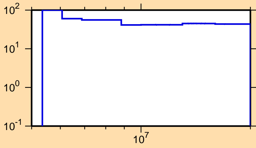
\Delta\sigma/\sigma vs. E for ^{73}\text{Kr}(n,ncont.)
