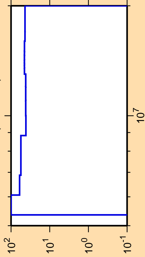
\Delta\sigma/\sigma vs. E for ^{73}\text{Kr}(n,\text{ncont.})
