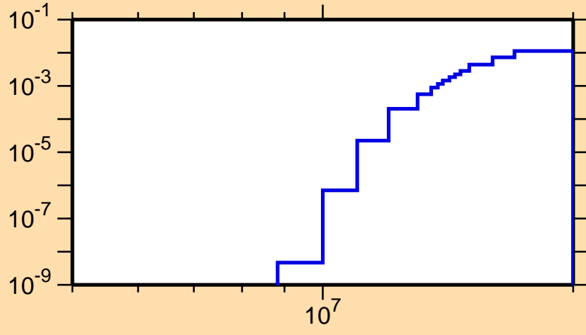
\sigma vs. E for ^{73}\text{Kr}(n,pd)
