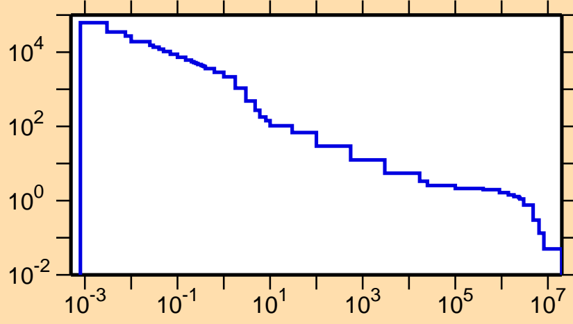
\sigma vs. E for ^{73}\text{Kr}(n,p)
