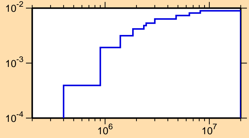
\sigma vs. E for ^{73}\text{Kr}(n,n_4)
