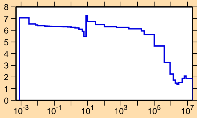
\sigma vs. E for ^{73}\text{Kr}(n,\text{el.})
