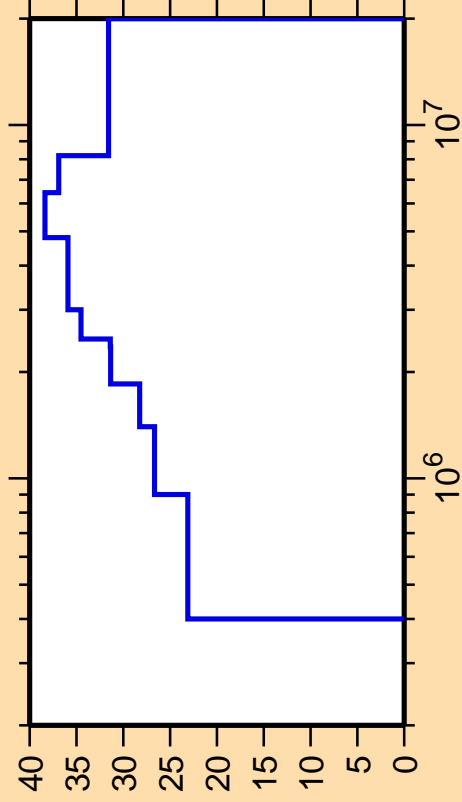
\Delta\sigma/\sigma vs. E for ^{73}\text{Kr}(n,n_4)
