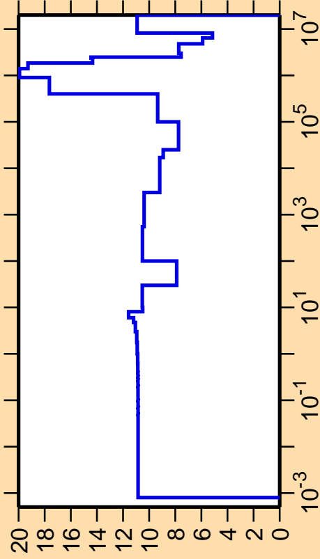
\Delta\sigma/\sigma vs. E for ^{73}\text{Kr}(n,\text{el.})
