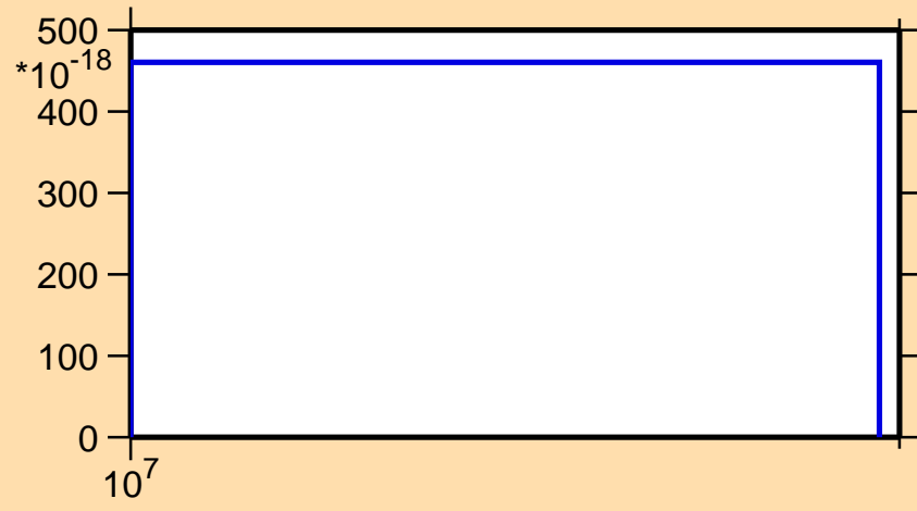
\sigma vs. E for ^{74}\text{Kr}(n,2np)
