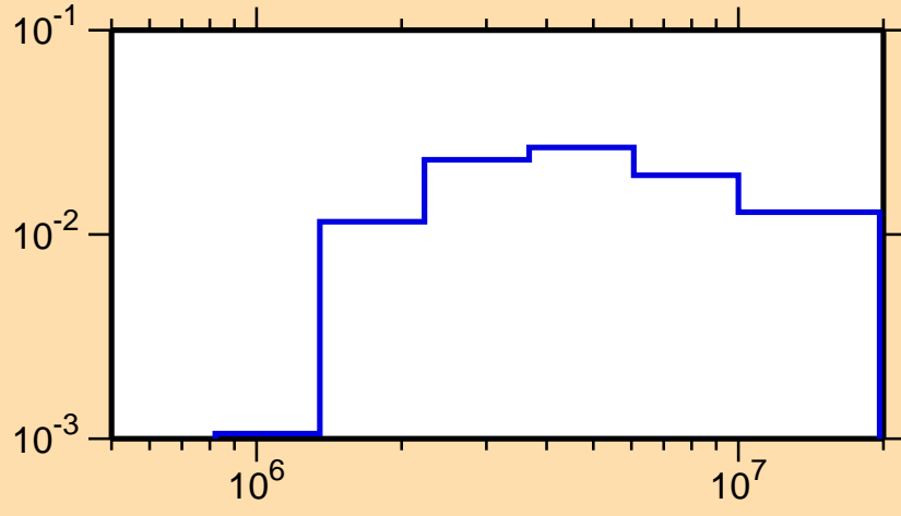
\sigma vs. E for ^{74}\text{Kr}(n,n_3)
