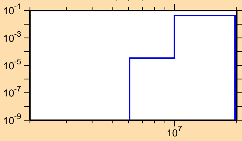
\sigma vs. E for ^{74}\text{Kr}(n,p\alpha)
