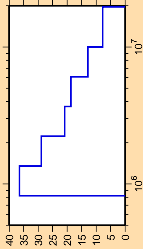
\Delta\sigma/\sigma vs. E for ^{74}\text{Kr}(n,n_3)
