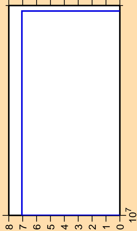
\Delta\sigma/\sigma vs. E for ^{74}\text{Kr}(n,n_1)
