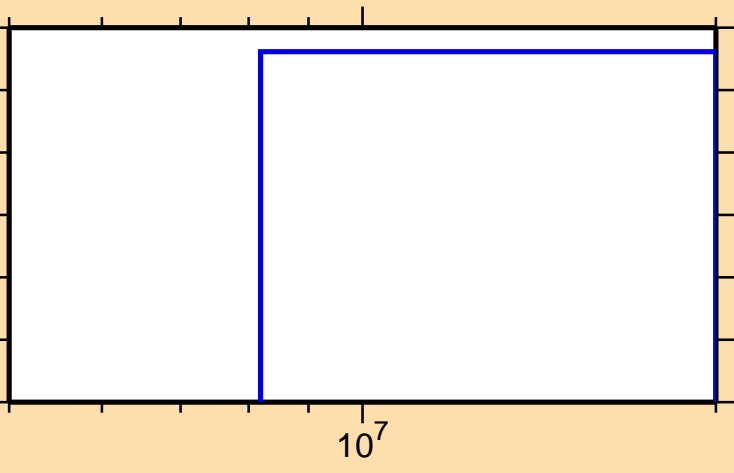
\sigma vs. E for ^{74}\text{Kr}(\text{mt } 45)
