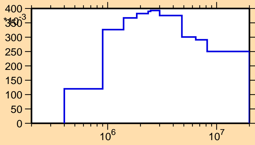
\sigma vs. E for ^{74}\text{Kr}(n,\text{inel.})
