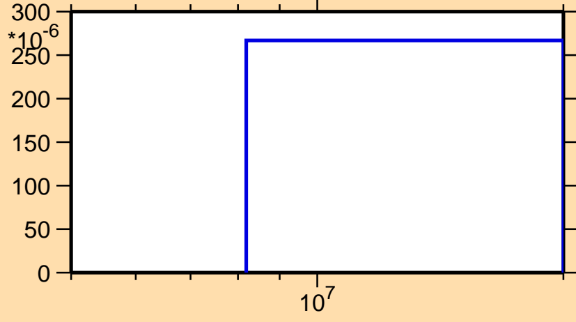
\sigma vs. E for ^{74}\text{Kr}(n,\text{pd})
