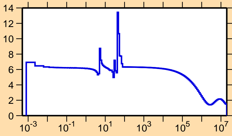
\sigma vs. E for ^{75}\text{Kr}(n,\text{el.})
