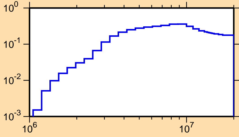
\sigma vs. E for ^{75}\text{Kr}(n,n\text{cont.})
