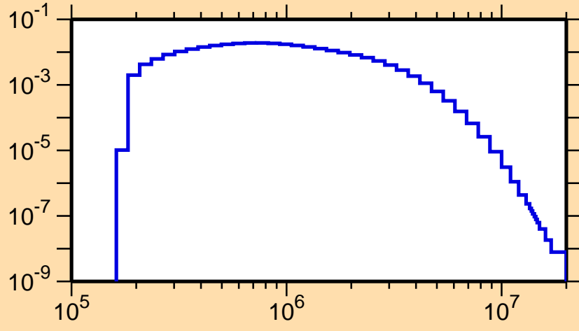
\sigma vs. E for ^{75}\text{Kr}(n,n_1)
