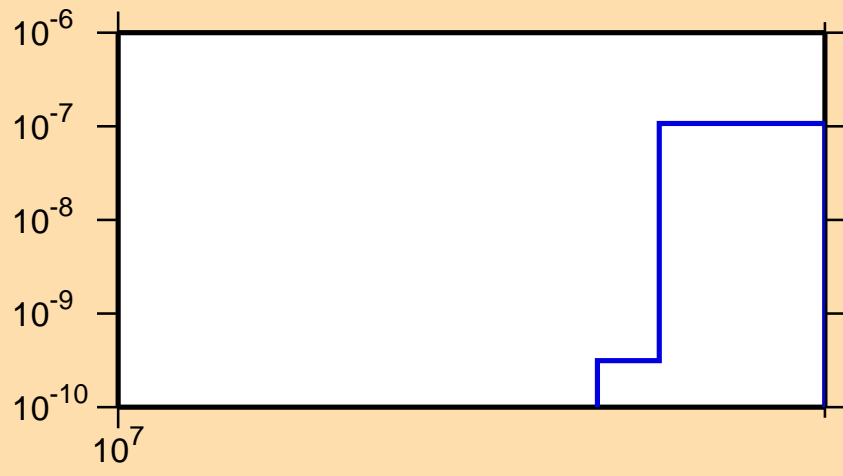
\sigma vs. E for ^{75}\text{Kr} (mt 45)
