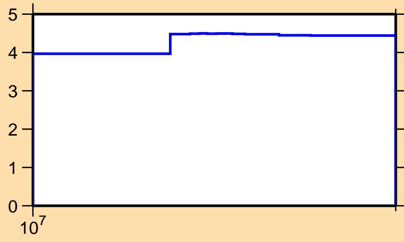
\Delta\sigma/\sigma vs. E for ^{75}\text{Kr}(n,\text{tot.})
