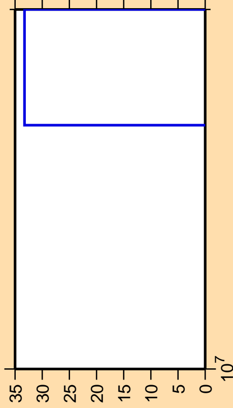
\Delta\sigma/\sigma vs. E for ^{75}\text{Kr} (mt 45)
