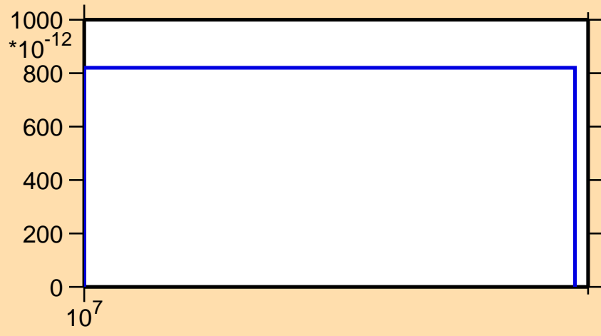
\sigma vs. E for ^{75}\text{Kr} (mt 45)
