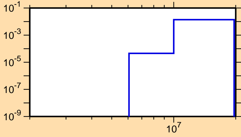
\sigma vs. E for ^{75}\text{Kr}(n,d)
