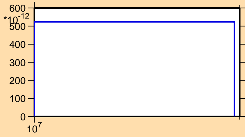
\sigma vs. E for ^{75}\text{Kr} (mt 34)
