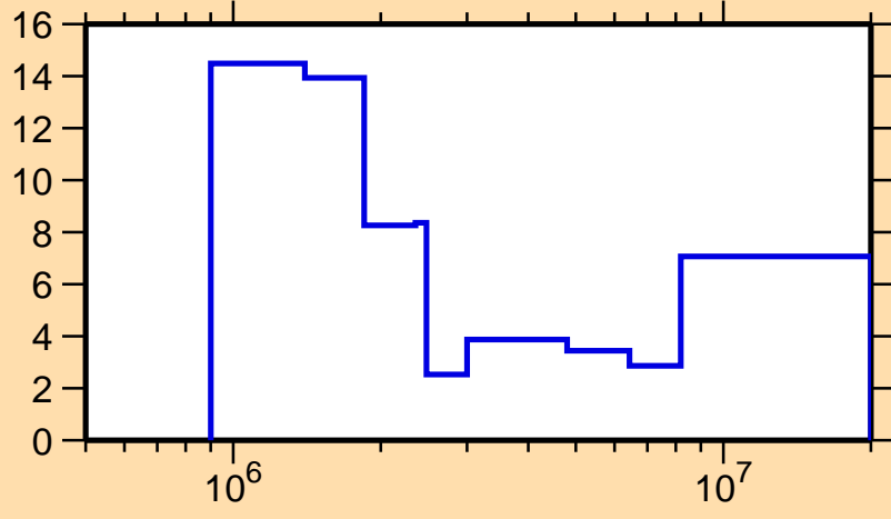
\Delta\sigma/\sigma vs. E for ^{75}\text{Kr}(n, el.)
