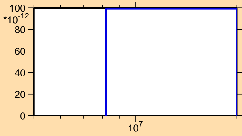
\sigma vs. E for ^{75}\text{Kr}(\text{mt117})
