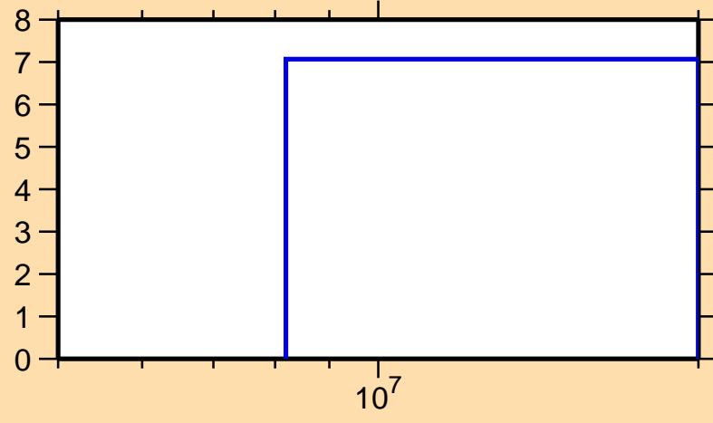
\Delta\sigma/\sigma vs. E for ^{75}\text{Kr}(n,\text{el.})
