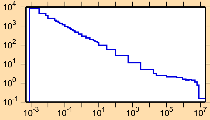
\sigma vs. E for ^{75}\text{Kr}(n,p)
