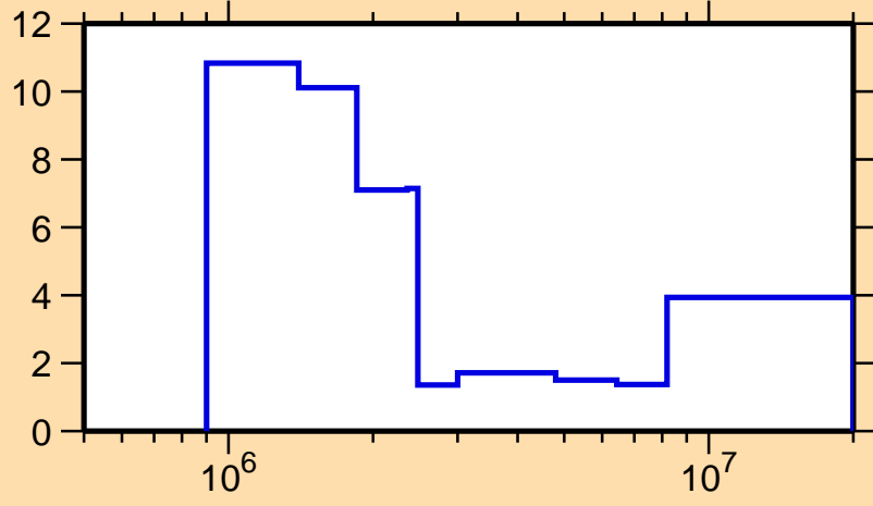
\Delta\sigma/\sigma vs. E for ^{75}\text{Kr}(n,tot.)
