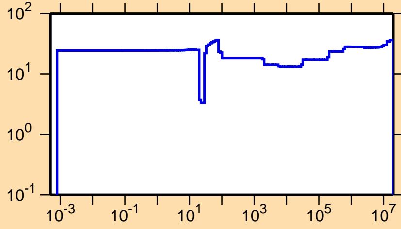
\Delta\sigma/\sigma vs. E for ^{76}\text{Kr}(n,\gamma)
