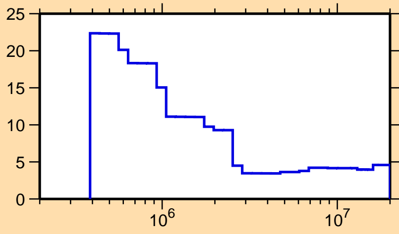
\Delta\sigma/\sigma vs. E for ^{76}\text{Kr}(n,\text{nonel.})
