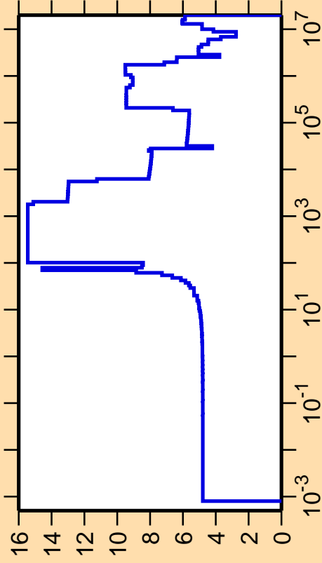
\Delta\sigma/\sigma vs. E for ^{76}\text{Kr}(n,\text{el.})
