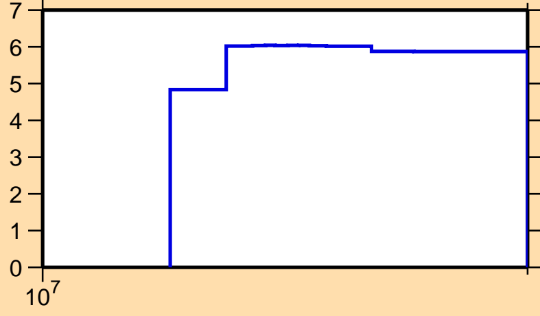
\Delta\sigma/\sigma vs. E for ^{76}\text{Kr}(n,\text{el.})
