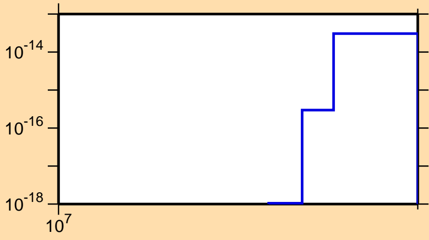
\sigma vs. E for ^{76}\text{Kr} (mt 34)
