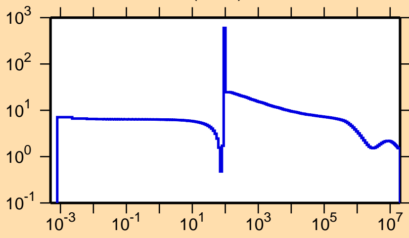
\sigma vs. E for ^{76}\text{Kr}(n,\text{el.})
