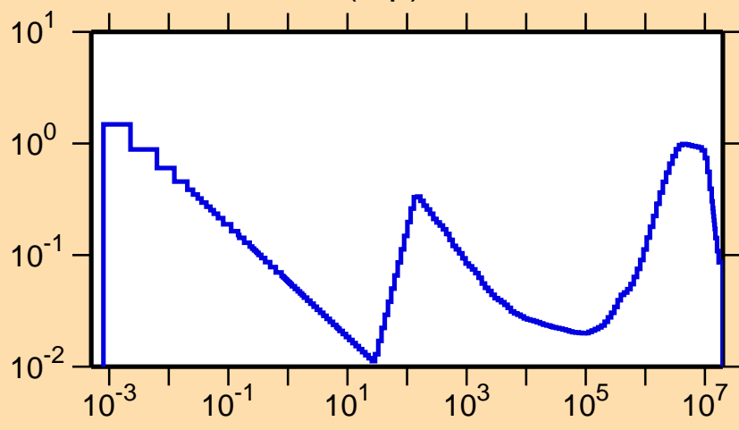
\sigma vs. E for ^{76}\text{Kr}(n,p)
