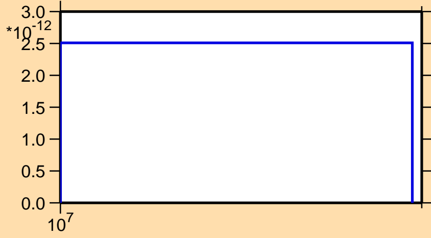
\sigma vs. E for ^{76}\text{Kr}(n,\text{nd})
