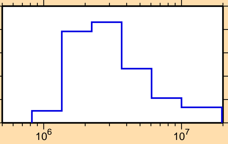
\sigma vs. E for ^{76}\text{Kr}(n,n_3)
