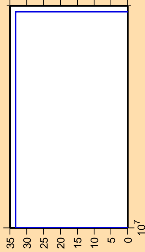
\Delta\sigma/\sigma vs. E for ^{76}\text{Kr} (mt 45)
