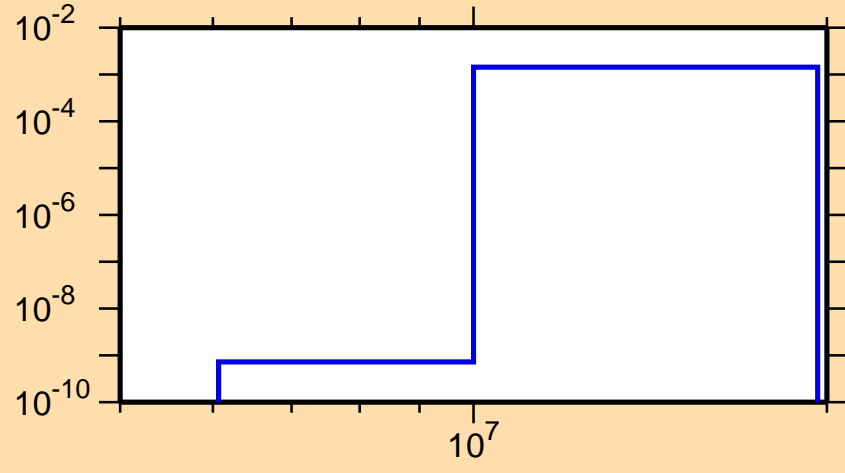
\sigma vs. E for ^{76}\text{Kr}(n,p\alpha)
