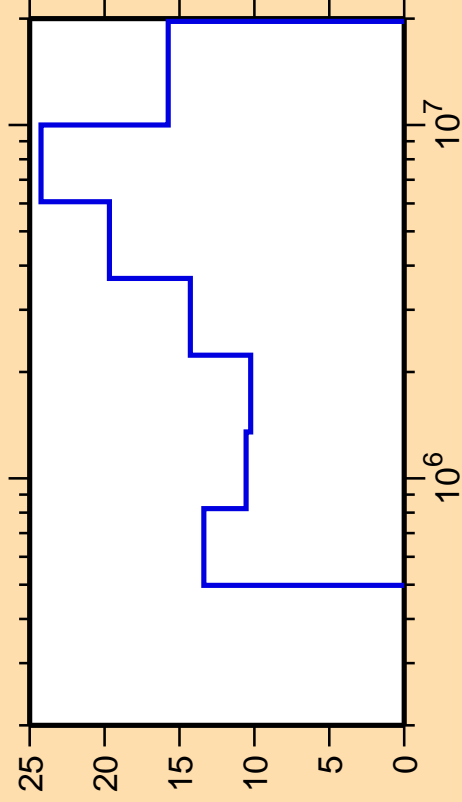
\Delta\sigma/\sigma vs. E for ^{76}\text{Kr}(n,n_2)
