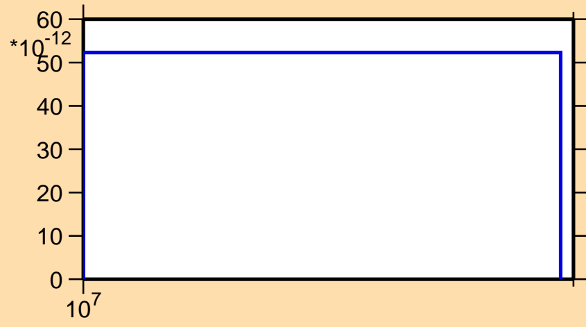
\sigma vs. E for ^{76}\text{Kr} (mt 45)
