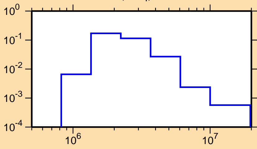
\sigma vs. E for ^{76}\text{Kr}(n,n_4)
