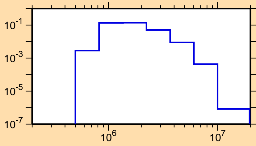
\sigma vs. E for ^{76}\text{Kr}(n,n_2)
