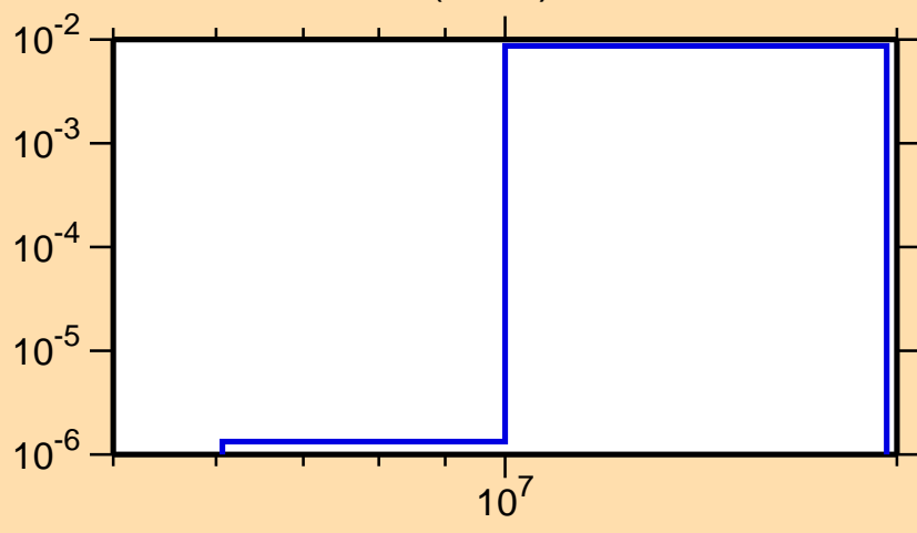
\sigma vs. E for ^{76}\text{Kr}(n,n\alpha)
