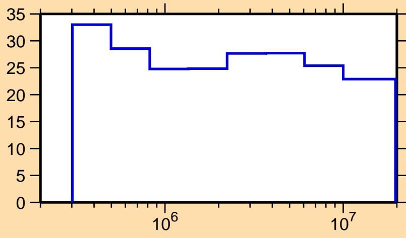
\Delta\sigma/\sigma vs. E for ^{76}\text{Kr}(n,n_1)
