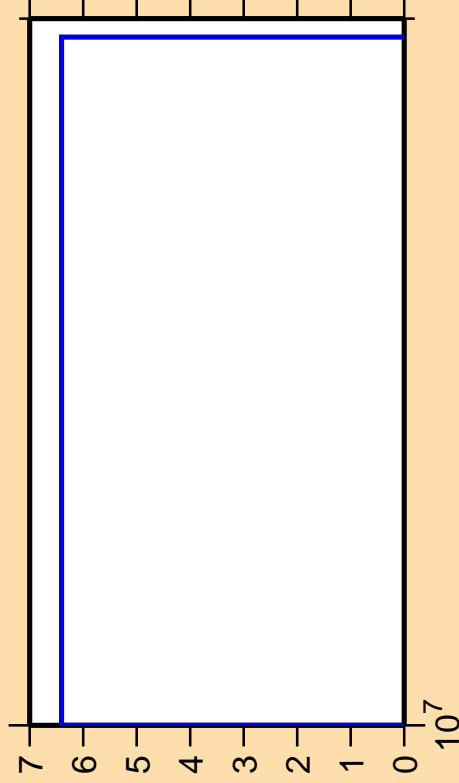
\Delta\sigma/\sigma vs. E for ^{76}\text{Kr}(n,\text{nd})
