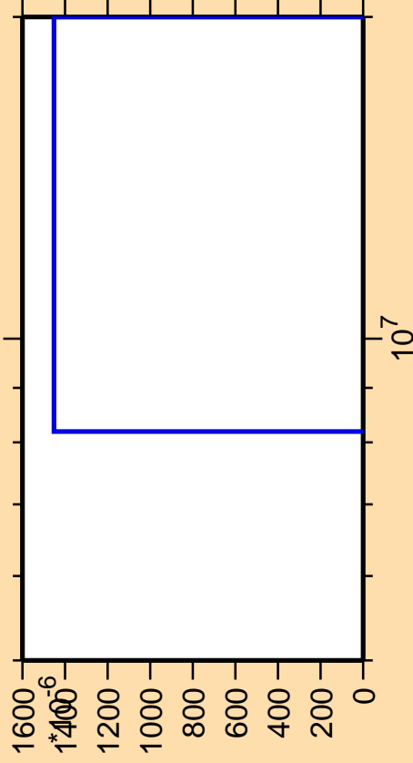
\Delta\sigma/\sigma vs. E for ^{76}\text{Kr}(\text{mt } 34)
