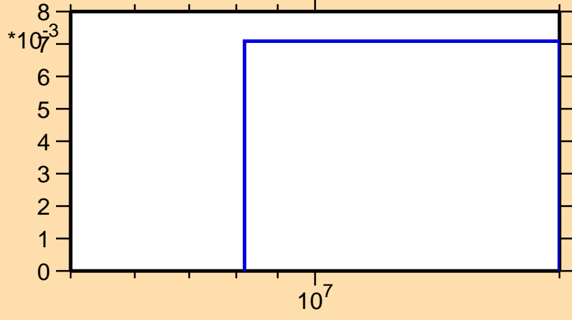
\sigma vs. E for ^{76}\text{Kr}(n,2n)
