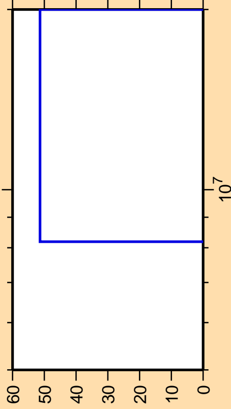
\Delta\sigma/\sigma vs. E for ^{76}\text{Kr}(n,2n)
