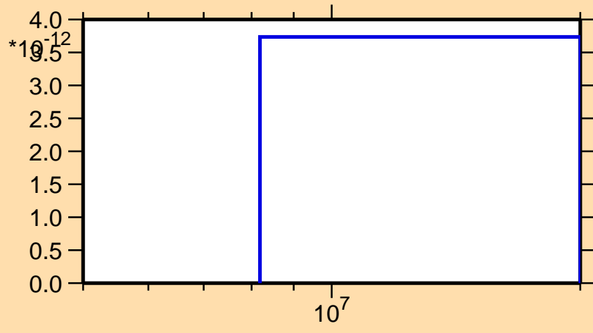
\sigma vs. E for ^{76}\text{Kr}(n,nd)
