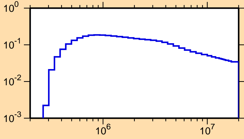
\sigma vs. E for ^{77}\text{Kr}(n,n_4)
