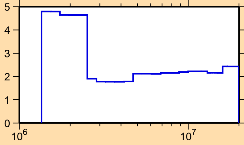
\Delta\sigma/\sigma vs. E for ^{77}\text{Kr}(n,n\text{onel.})
