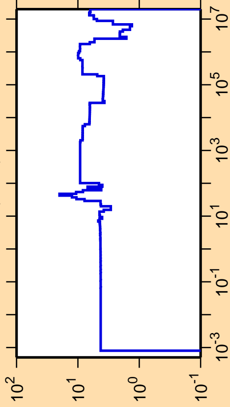
\Delta\sigma/\sigma vs. E for ^{77}\text{Kr}(n,\text{el.})
