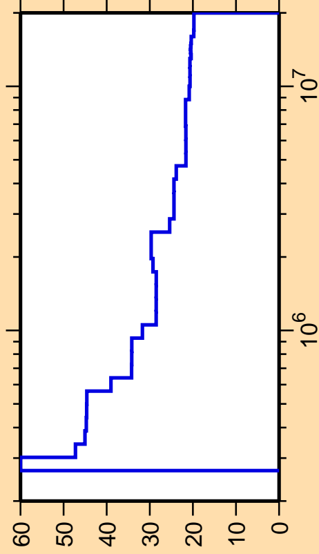
\Delta\sigma/\sigma vs. E for ^{77}\text{Kr}(n,n_4)
