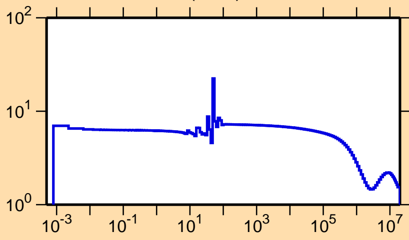
\sigma vs. E for ^{77}\text{Kr}(n,\text{el.})
