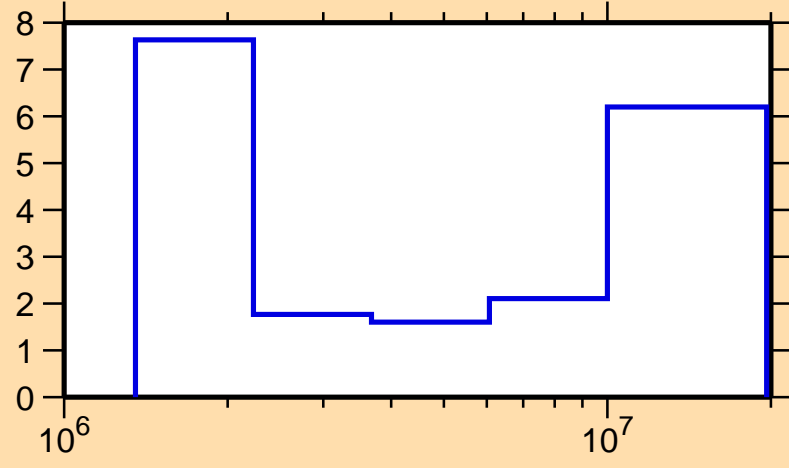
\Delta\sigma/\sigma vs. E for ^{77}\text{Kr}(n, el.)
