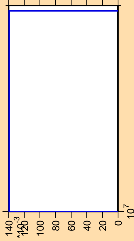
\Delta\sigma/\sigma vs. E for ^{77}\text{Kr} (mt 45)
