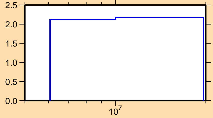
\Delta\sigma/\sigma vs. E for ^{77}\text{Kr}(n,\text{nonel.})
