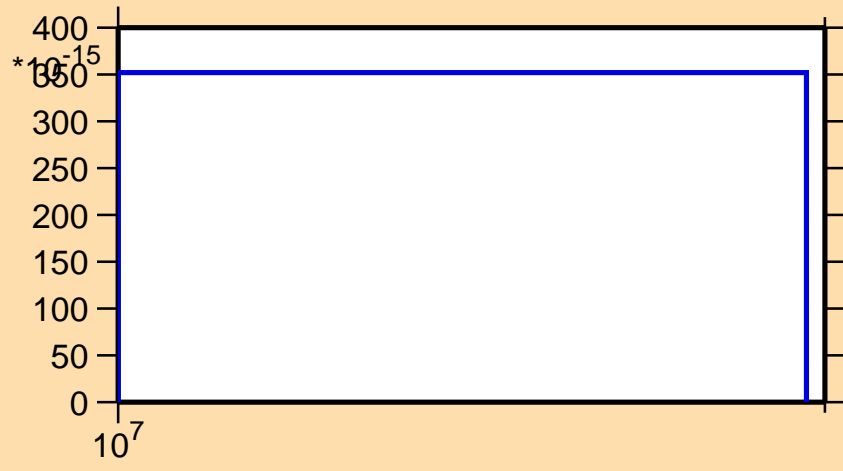
\sigma vs. E for ^{77}\text{Kr} (mt 45)
