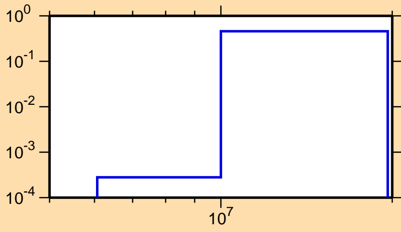
\sigma vs. E for ^{77}\text{Kr}(n,np)
