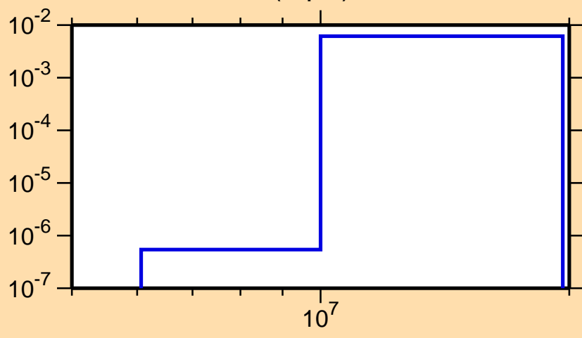
\sigma vs. E for ^{77}\text{Kr}(n,p\alpha)
