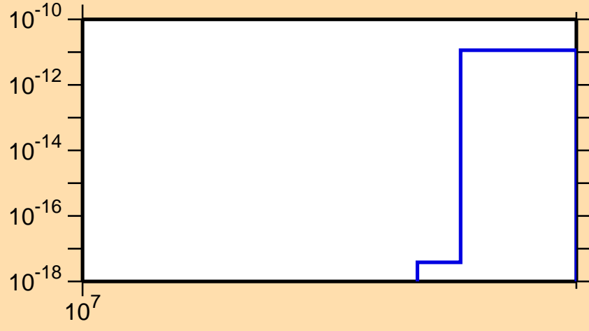
\sigma vs. E for ^{79}\text{Kr} (mt 34)
