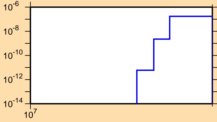
\sigma vs. E for ^{79}\text{Kr}(n,\text{pd})
