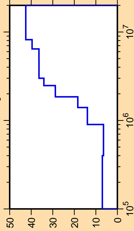
\Delta\sigma/\sigma vs. E for ^{79}\text{Kr}(n,n_3)
