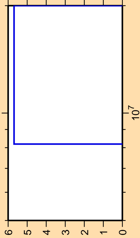
\Delta\sigma/\sigma vs. E for ^{79}\text{Kr}(n,n\text{cont.})
