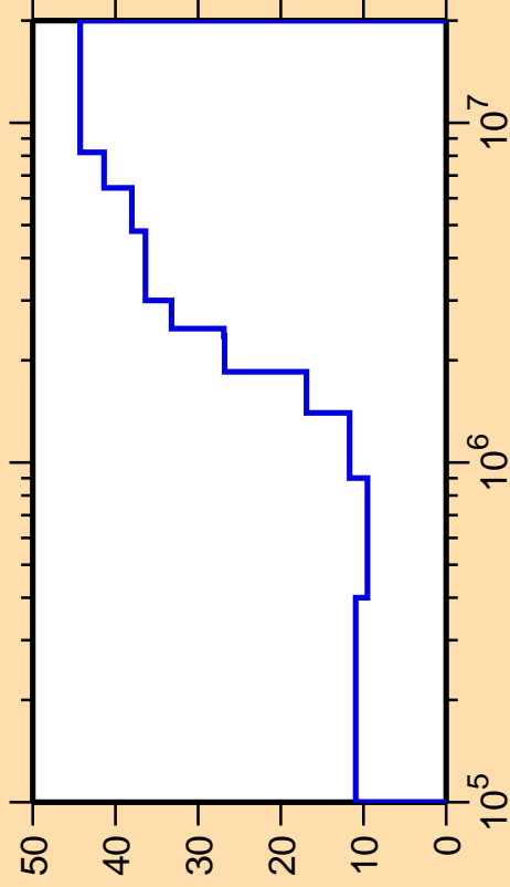
\Delta\sigma/\sigma vs. E for ^{79}\text{Kr}(n,n_4)
