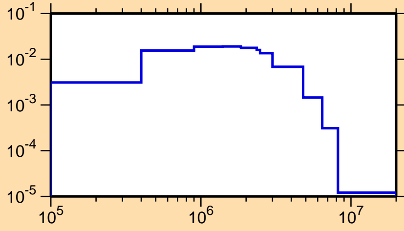
\sigma vs. E for ^{79}\text{Kr}(n,n_3)
